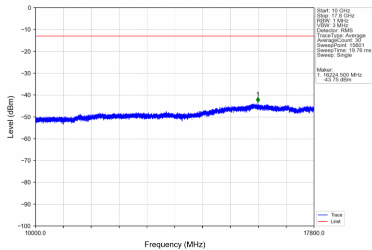
Band66_10MHz_QPSK_MCH_1745MHz_RB_1_0_NTNV
