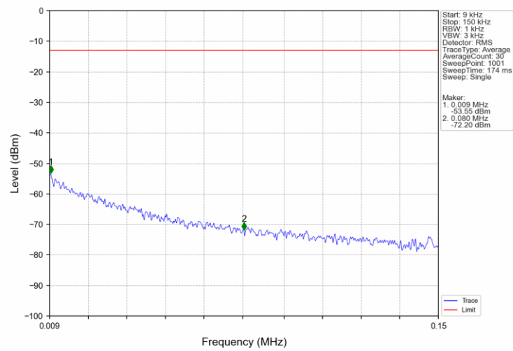
Band66 10MHz 16QAM MCH 1745MHz RB 1 0 NTNV
