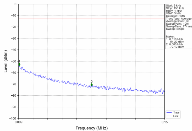
Band66 15MHz 16QAM MCH 1745MHz RB 1 0 NTN
