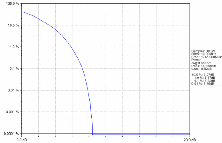
Band66_20MHz_16QAM_MCH_1745MHz_RB_27_0_NTNV
