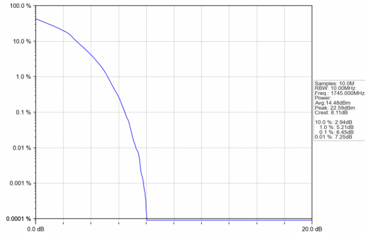
Band66_10MHz_16QAM_MCH_1745MHz_RB_27_0_NTNV
