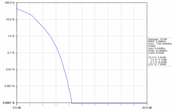
Band66_5MHz_16QAM_MCH_1745MHz_RB_25_0_NTNV
