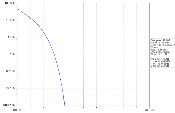
Band66_10MHz_QPSK_LCH_1715MHz_RB_50_0_NTNV
