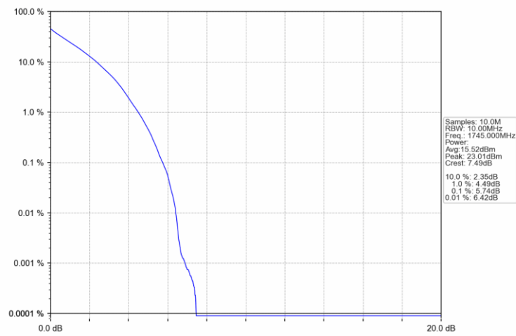
Band66_10MHz_QPSK_MCH_1745MHz_RB_50_0_NTNV
