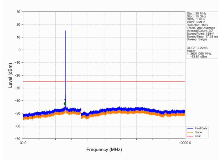
Band41_15MHz_16QAM_HCH_2647.5MHz_RB_1_0_NTNV
