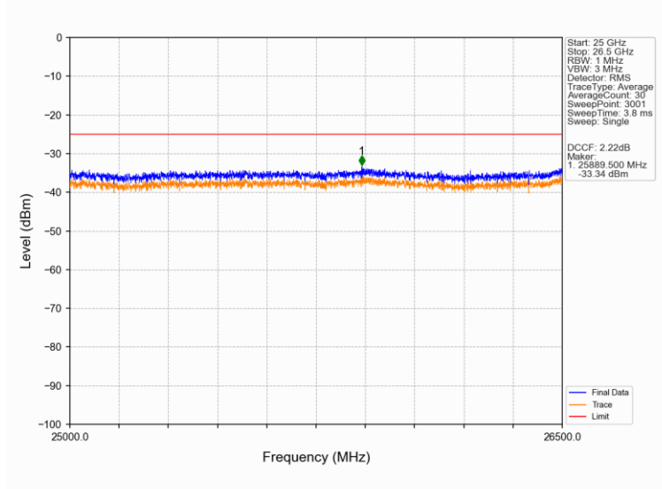
Band41_15MHz_16QAM_MCH_2605MHz_RB_1_0_NTNV
