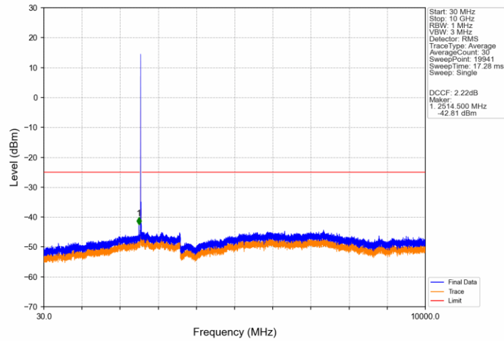
Band41 15MHz 16QAM LCH 2562.5MHz RB 1 0 NTNV
