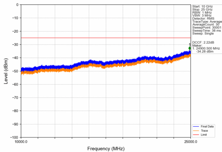
Band41 15MHz 16QAM LCH 2562.5MHz RB 1 0 NTNV
