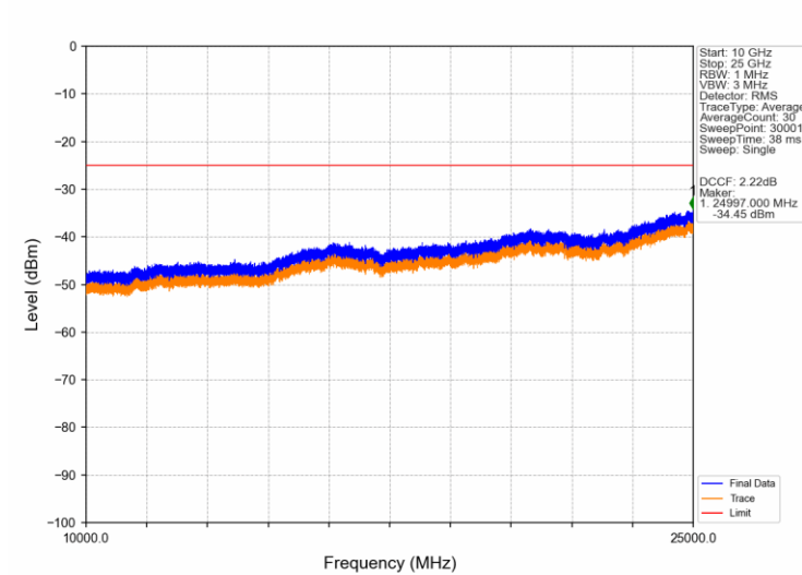
Band41_15MHz_16QAM_HCH_2647.5MHz_RB_1_0_NTNV
