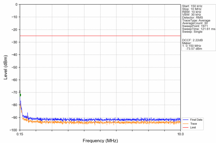
Band41_15MHz_16QAM_LCH_2562.5MHz_RB_1_0_NTNV
