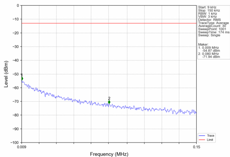
Band17 10MHz 16QAM MCH 710MHz RB 1 0 NTNV
