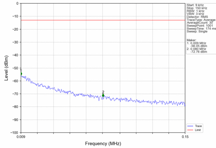
Band5 5MHz 16QAM HCH 846.5MHz RB 1 0 NTNV
