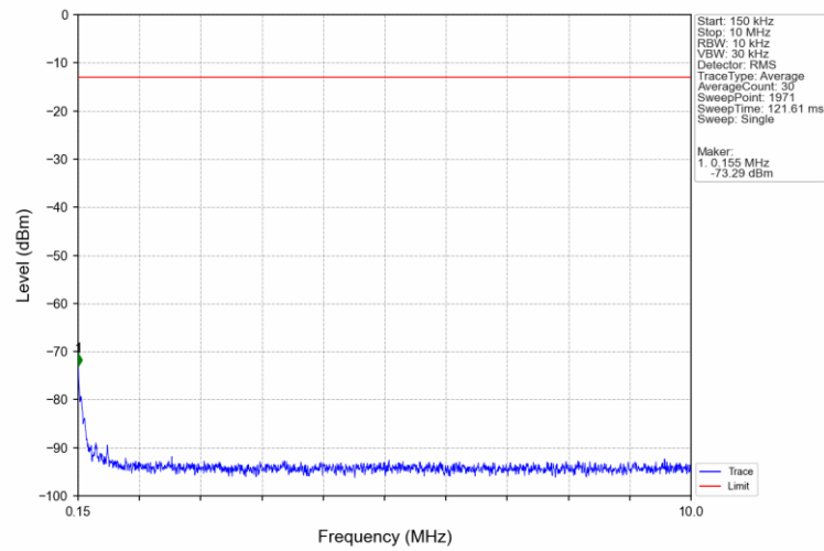
Band5 5MHz 16QAM HCH 846.5MHz RB 1 0 NTNV
