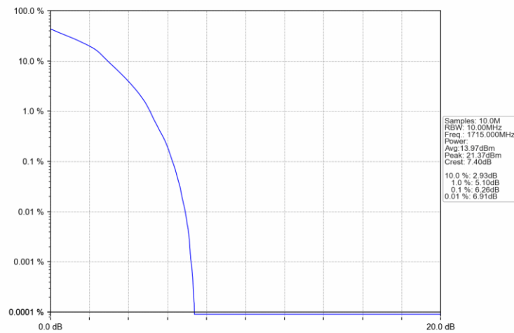
Band4 10MHz 16QAM LCH 1715MHz RB 27 0 NTNV
