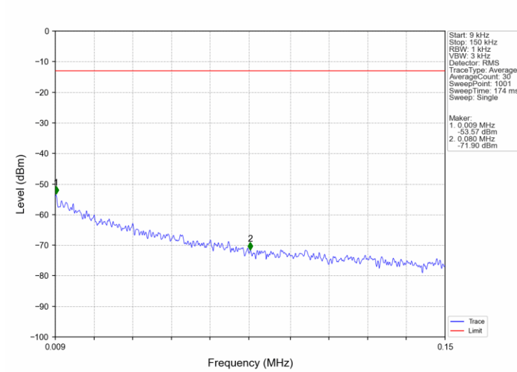
Band4 1.4MHz 16QAM HCH 1754.3MHz RB 1 0 NTN
