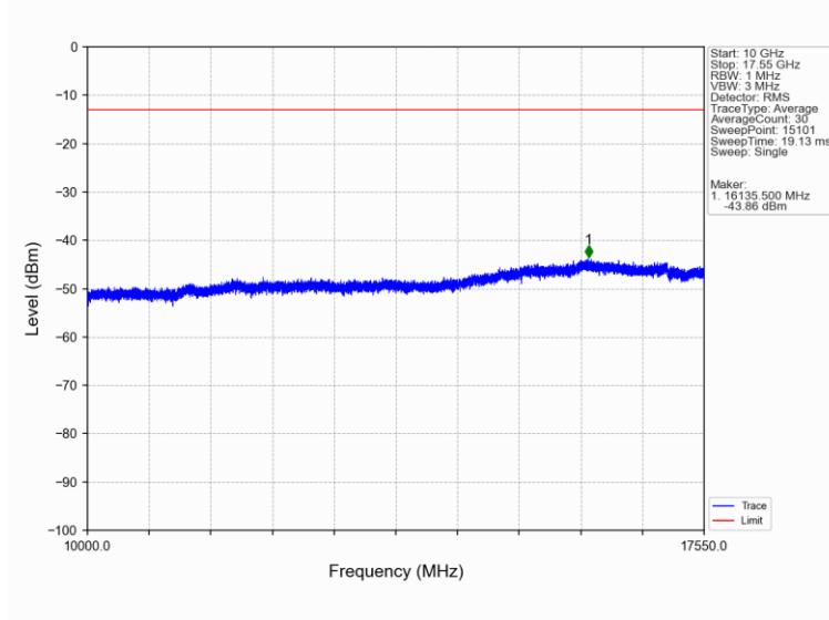
Band4 1.4MHz 16QAM HCH 1754.3MHz RB 1 0 NTN
