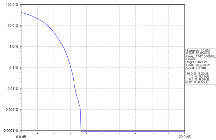
Band4 15MHz 16QAM HCH 1747.5MHz RB 27 48 NTN
