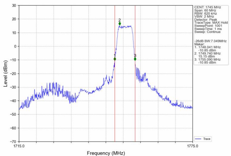
Band4 20MHz 16QAM HCH 1745MHz RB 27 73 NTN
