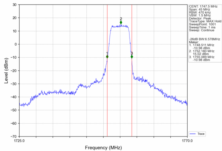
Band4 15MHz 16QAM HCH 1747.5MHz RB 27 48 NTN
