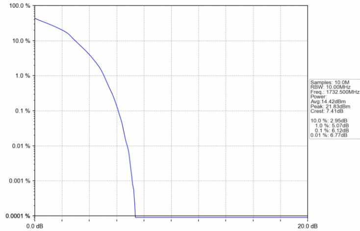
Band4 10MHz 16QAM MCH 1732.5MHz RB 27 0 NTN
