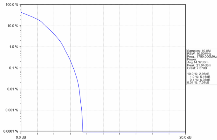
Band4 10MHz 16QAM HCH 1750MHz RB 27 23 NTN
