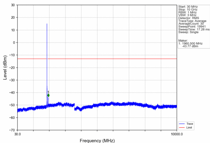
Band2 15MHz 16QAM MCH 1880MHz RB 1 0 NTV
