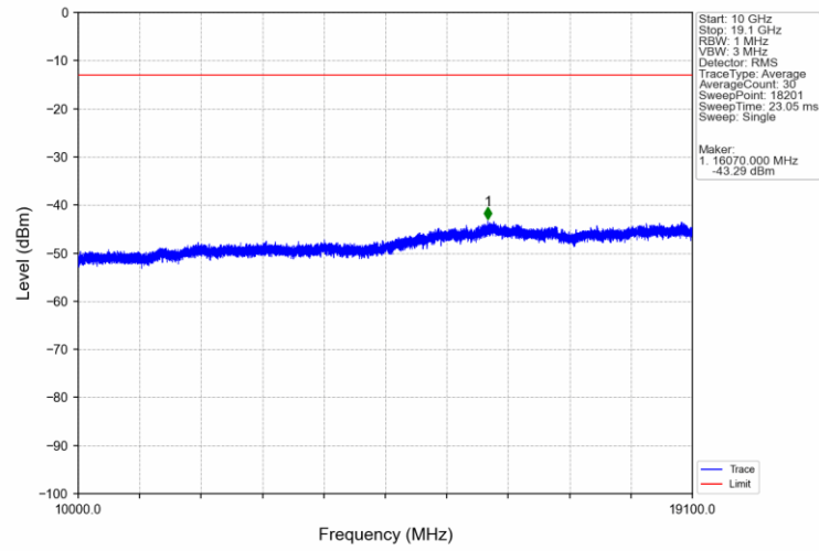
Band2_15MHz_16QAM_MCH_1880MHz_RB_1_0_NTNV
