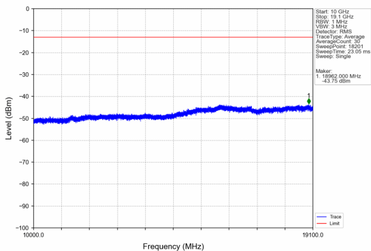
Band2 15MHz 16QAM MCH 1880MHz RB 1 0 NTV
