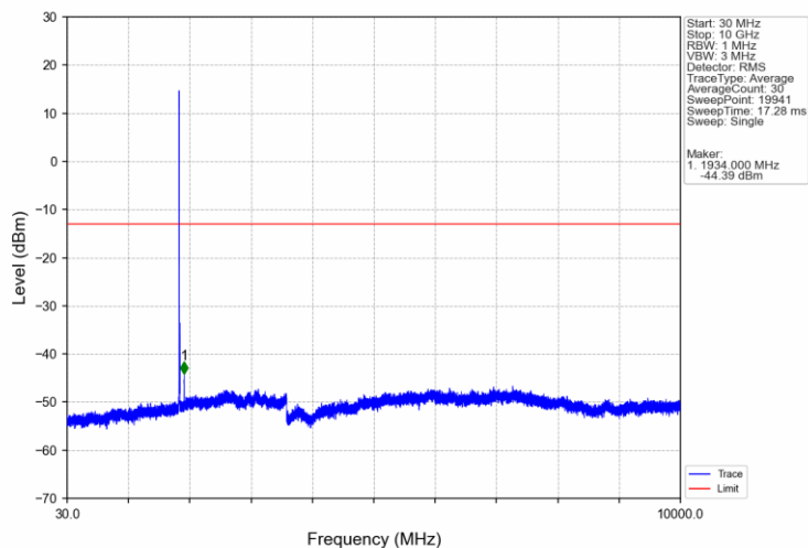
Band2_5MHz_QPSK_LCH_1852.5MHz_RB_1_0_NTNV
