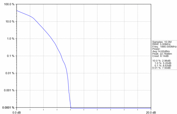
Band2 3MHz 16QAM MCH 1880MHz RB 15 0 NTV
