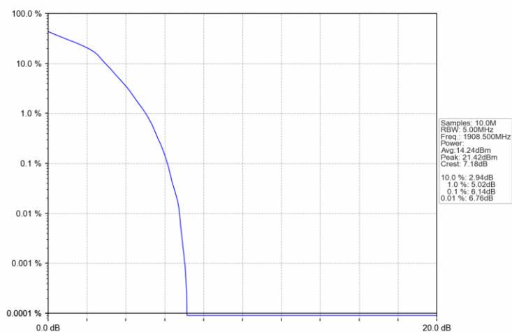
Band2 3MHz 16QAM HCH 1908.5MHz RB 15 0 NTV
