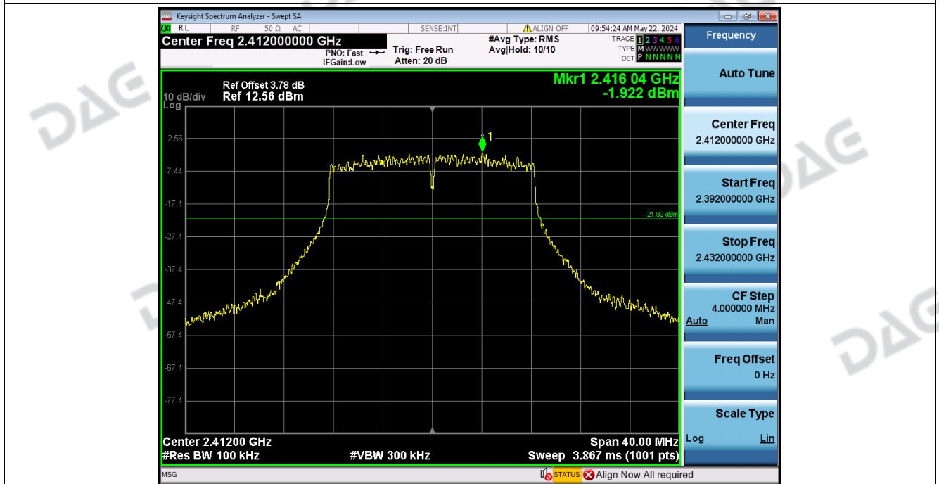
2_Bandedge_NVNT_ANT1_802_11g_2412
