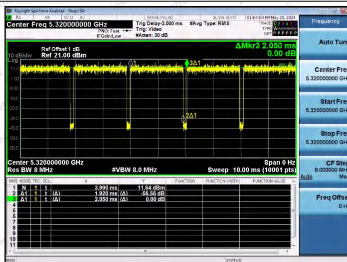
NTVN-11N20SISO-Ant1-5320
