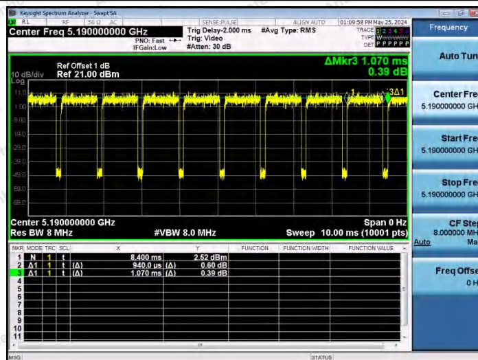
NTNV-11N40SISO-Ant1-5190
