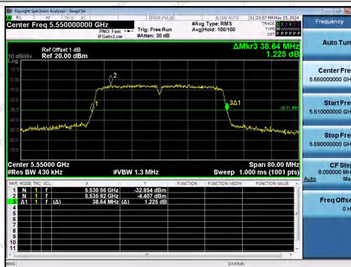
11N40SISO-Ant1-5550
