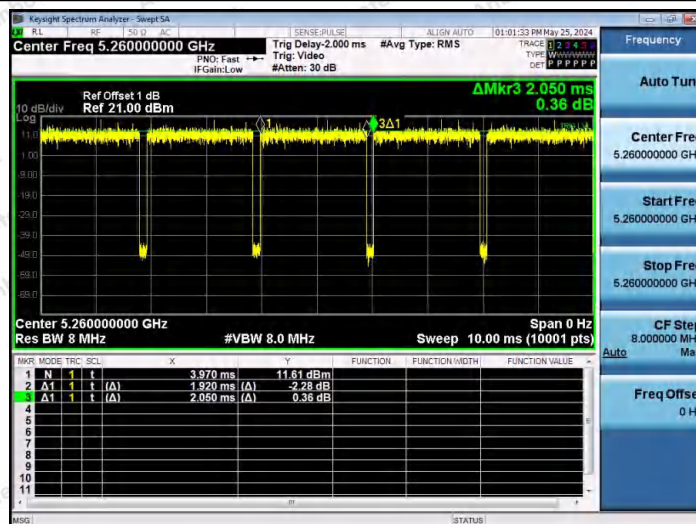
NTVN-11N20SISO-Ant1-5260
