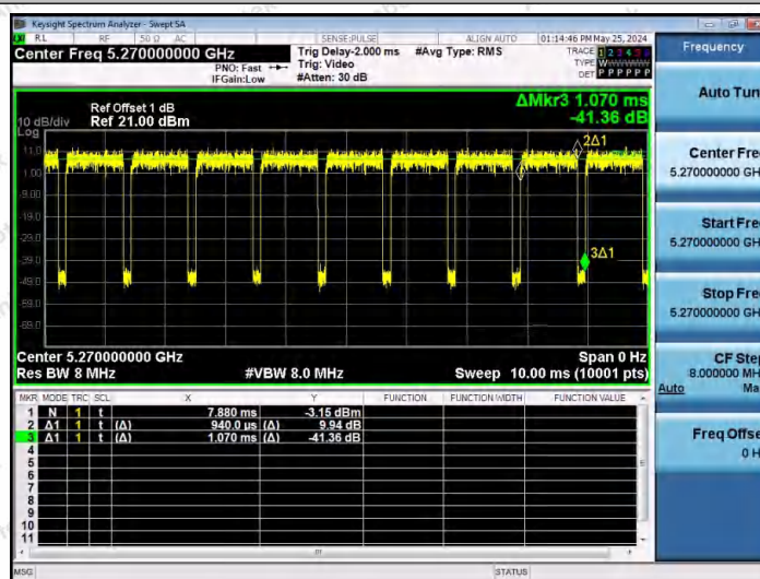
NTNV-11N40SISO-Ant1-5270
