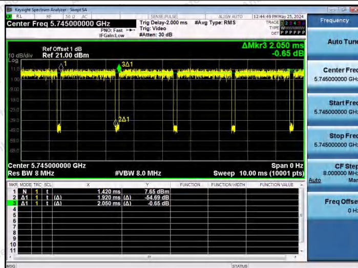
NTVN-11N20SISO-Ant1-5745
