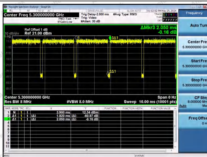
NTVN-11N20SISO-Ant1-5300
