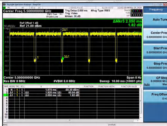
NTNV-11N20SISO-Ant1-5500
