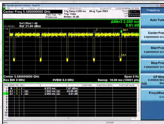
NTNV-11N20SISO-Ant1-5580
