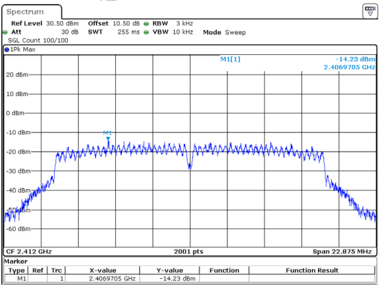
802.11g_2412MHz -14.23dBm/3kHz
