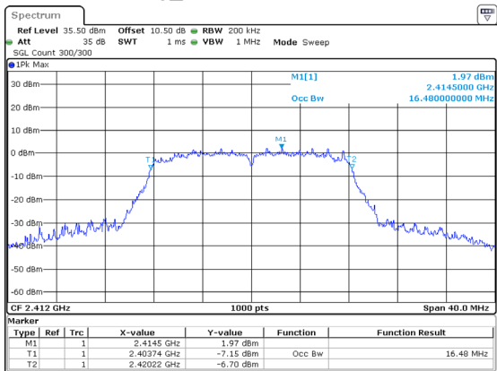
802.11g_2412MHz 16.480MHz
