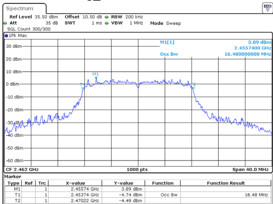
802.11g_2462MHz 16.480MHz
