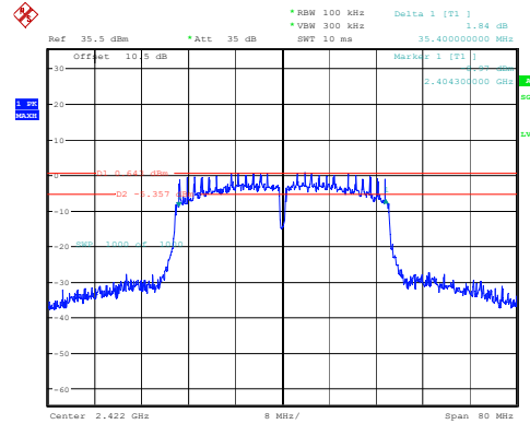
802.11n40_2422MHz 35.400MHz
