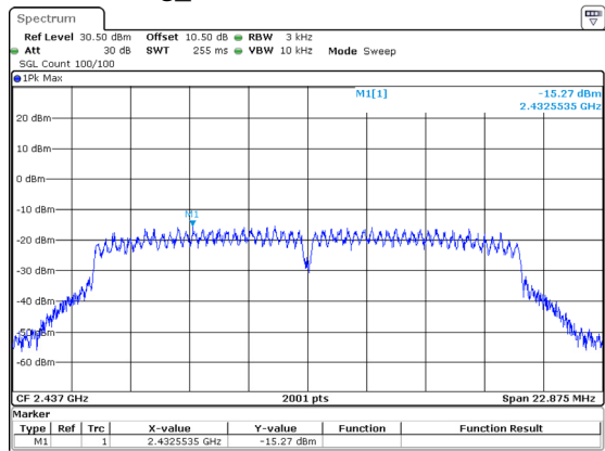
802.11g_2437MHz -15.27dBm/3kHz
