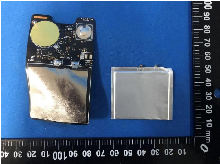
Battery 1(silver)
