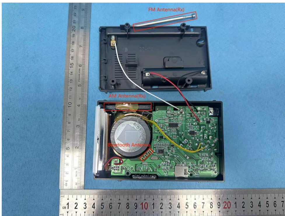
Internal Photos
