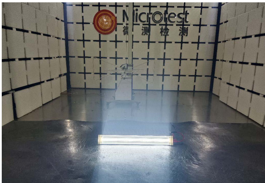
Radiated emissions (above 1GHz)
