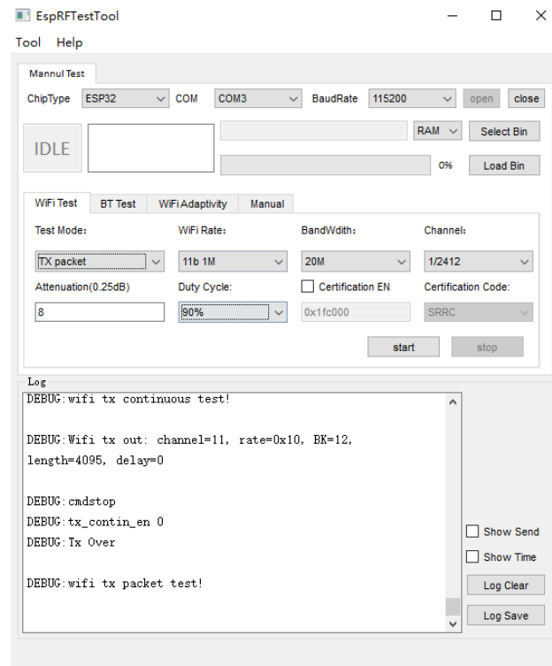
Software Setting Diagram
