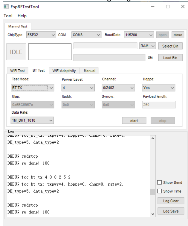
Software Setting Diagram
