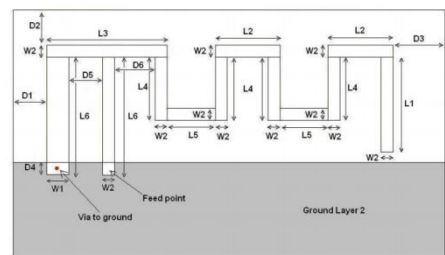
Figure 3: Antenna Dimensions https://www.researchgate.net/publication/351111111
