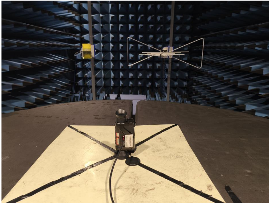
Radiated Emission Above 1GHz -Front
