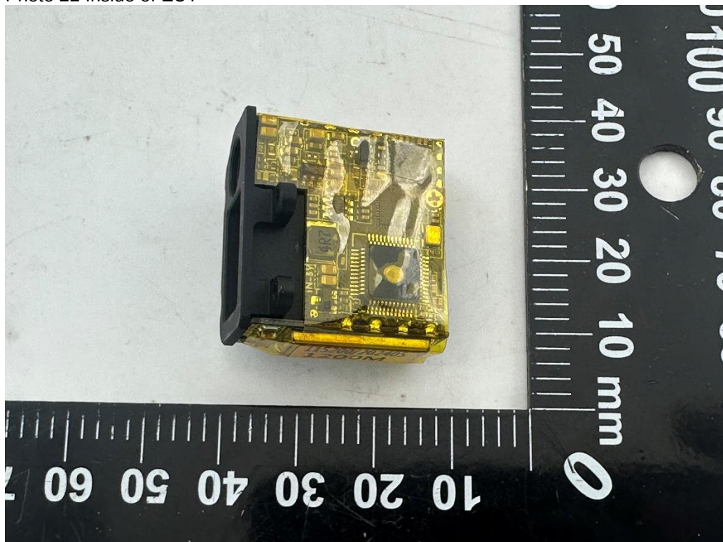
Photo 22 Inside of EUT
