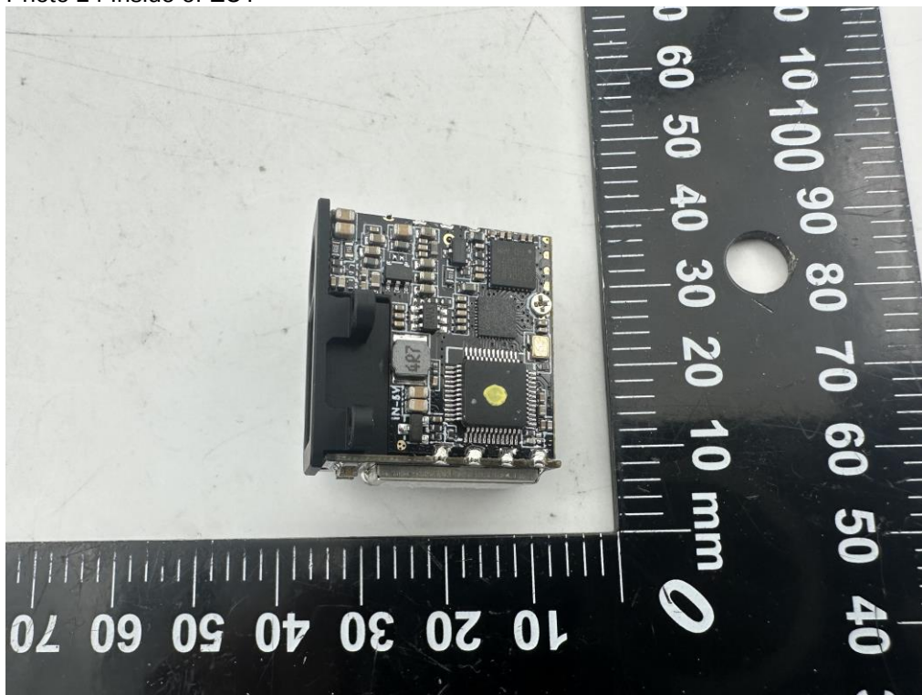
Photo 24 Inside of EUT
