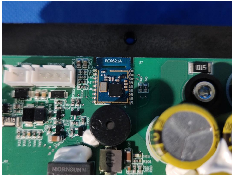
Antenna Location
