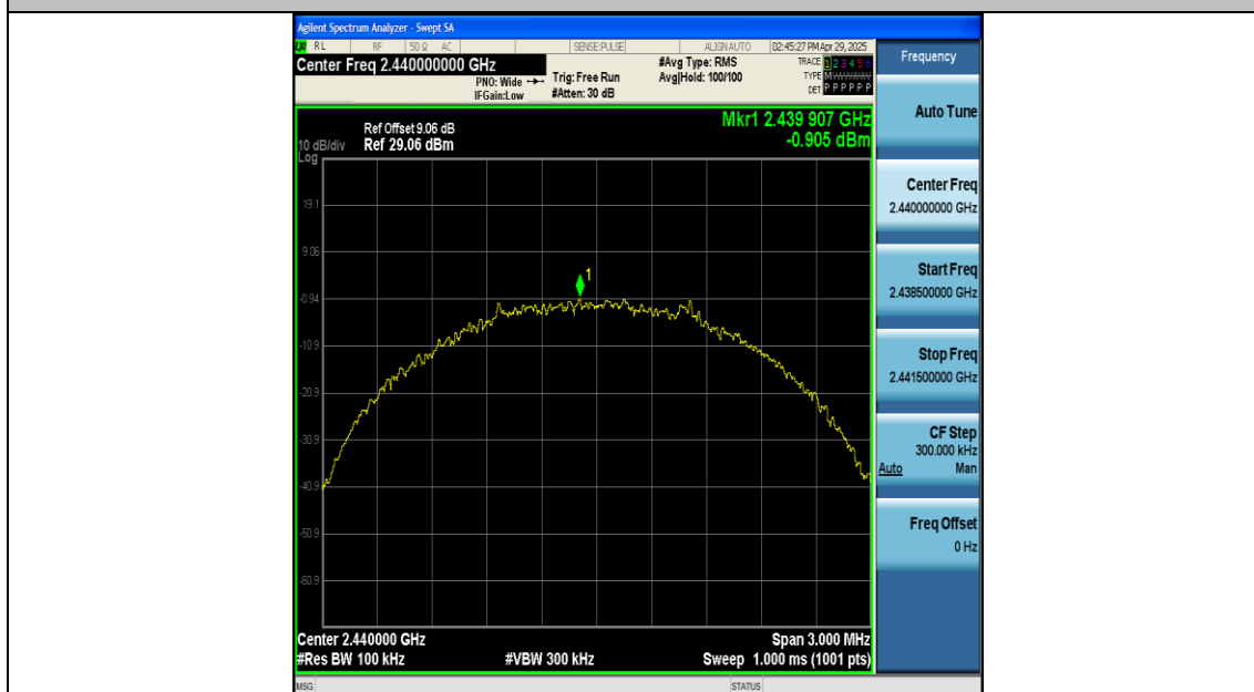
SRD-Ant1-2440-0~Reference-PASS
