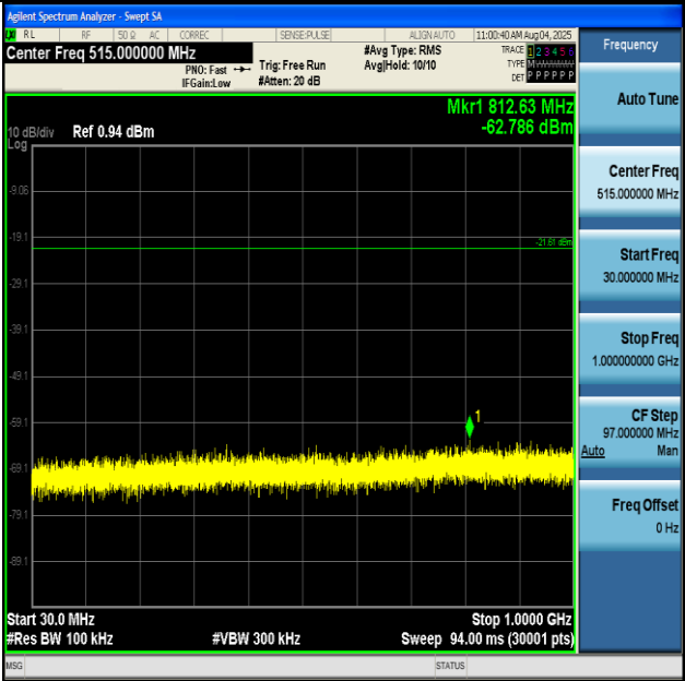
SRD-Ant1-2480-30~1000-PASS
