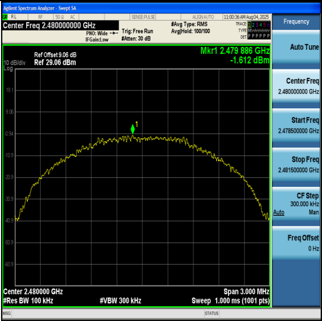
SRD-Ant1-2480-0~Reference-PASS
