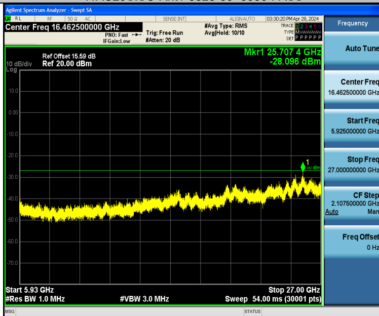
11AC20SISO-Ant1-5825-5925~27000-PASS
