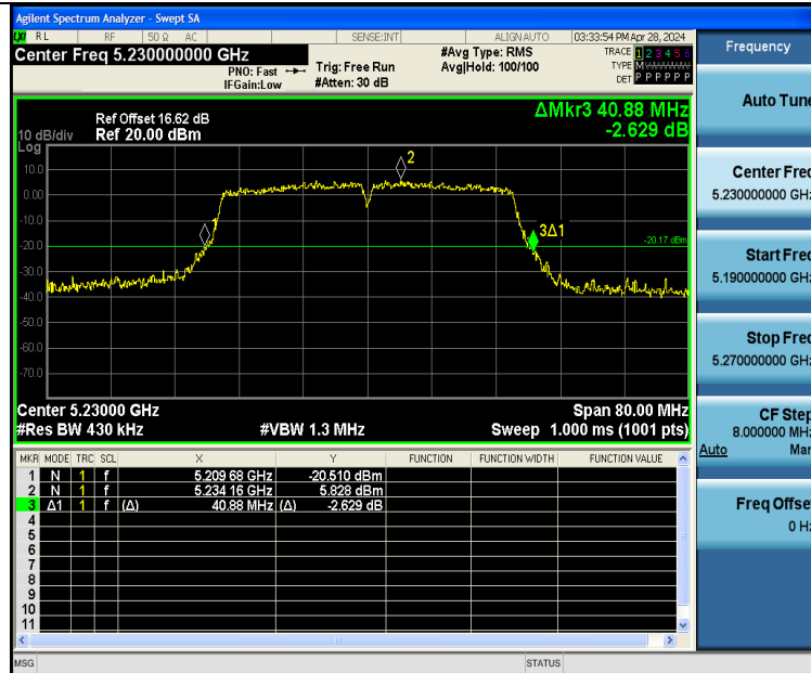
11AC40SISO-Ant1-5230
