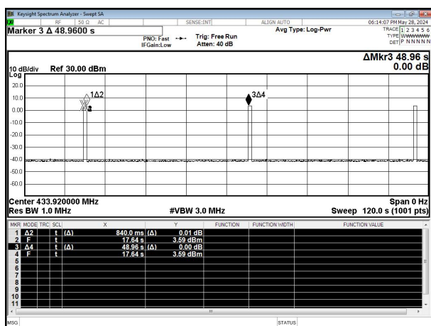
ASK 433.92MHz
