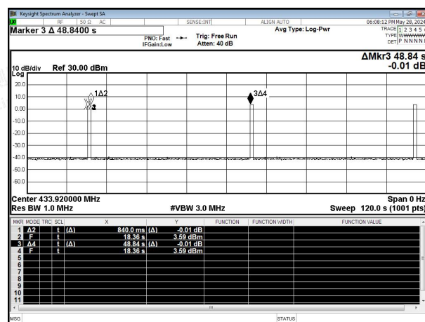
FSK 433.92MHz
