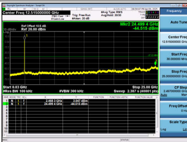
11BE20SISO-Ant4-2462-30~25000-PASS
