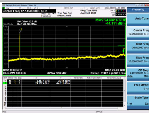
11AX40SISO-Ant4-2452-30~25000-PASS
