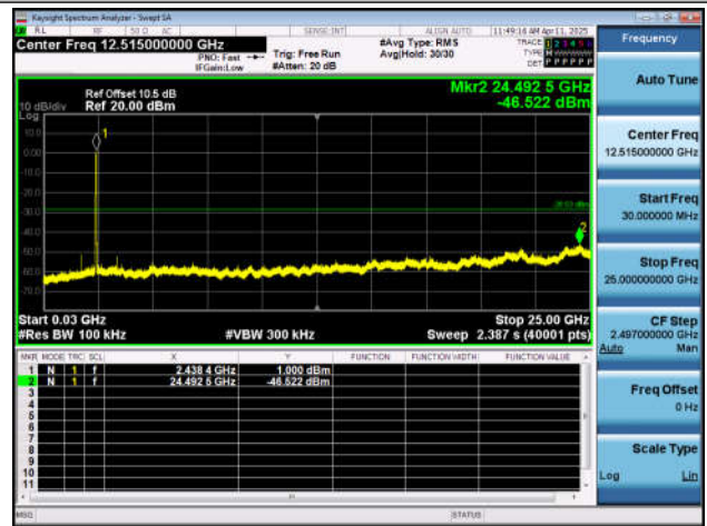
11AX40SISO-Ant7-2437-0~Reference-PASS
