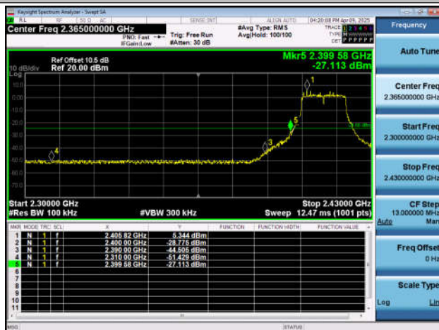
11G-Ant4-2412-PASS
