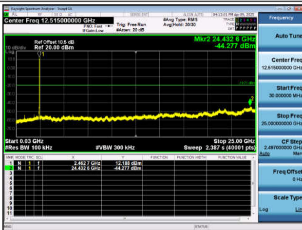
11B-Ant4-2462-30~25000-PASS
