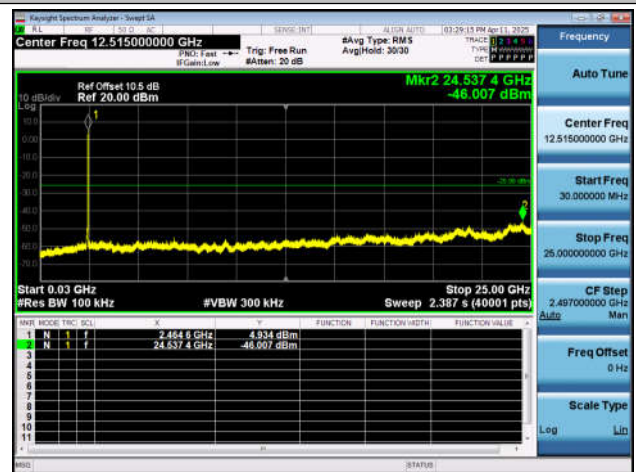
11BE20SISO-Ant7-2462-30~25000-PASS
