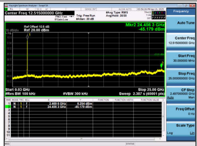
11G-Ant7-2462-30~25000-PASS
