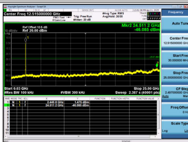
11AX40SISO-Ant7-2452-0~Reference-PASS
