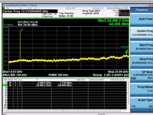
11AX40SISO-Ant4-2452-0~Reference-PASS
