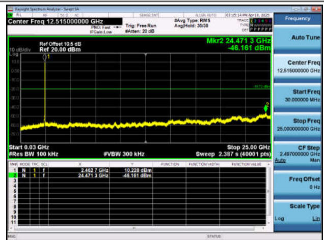
11B-Ant7-2462-30~25000-PASS
