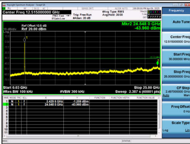
11BE40SISO-Ant4-2437-0~Reference-PASS
