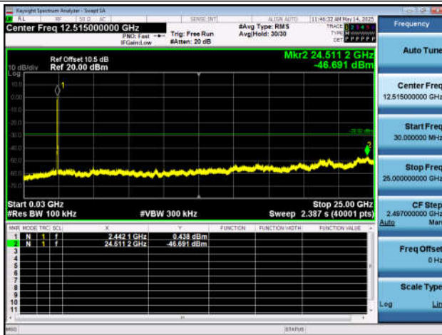
11N40SISO-Ant4-2452-0~Reference-PASS
