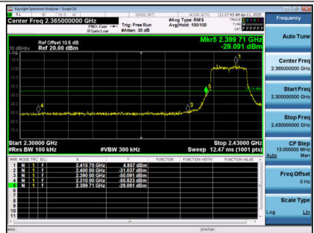
11AX20SISO-Ant7-2412-PASS
