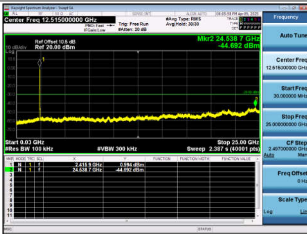
11AX40SISO-Ant4-2437-0~Reference-PASS
