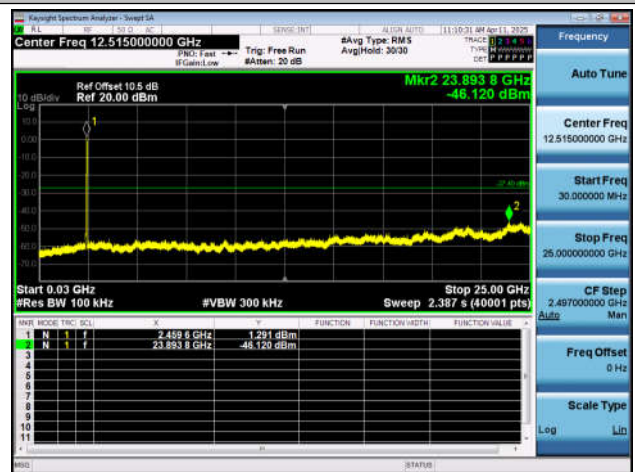
11N40SISO-Ant7-2452-30~25000-PASS
