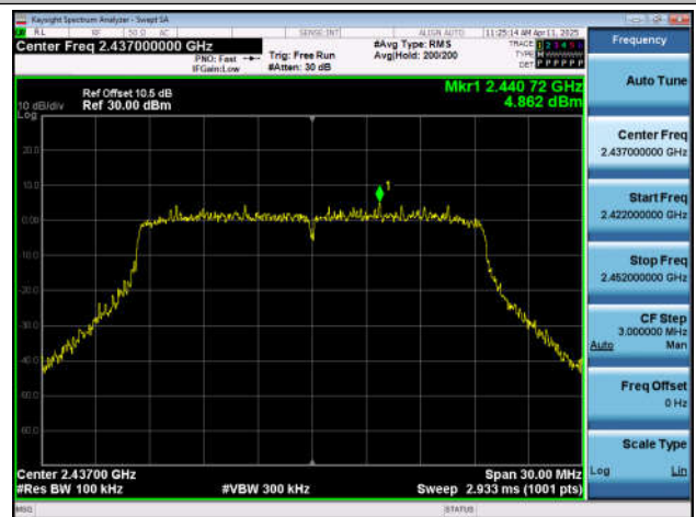
11AX20SISO-Ant7-2437-0~Reference-PASS
