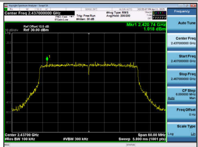
11BE40SISO-Ant7-2437-0~Reference-PASS
