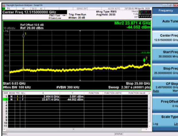
11AX20SISO-Ant4-2462-30~25000-PASS
