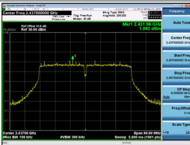
11N40SISO-Ant4-2437-0~Reference-PASS
