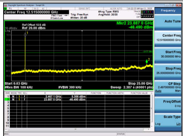
11N20SISO-Ant7-2462-30~25000-PASS
