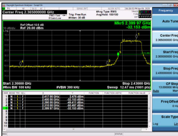
11AX20SISO-Ant4-2412-PASS
