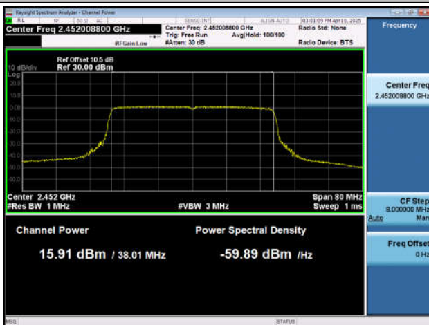
11BE40SISO-Ant4-2452-PASS
