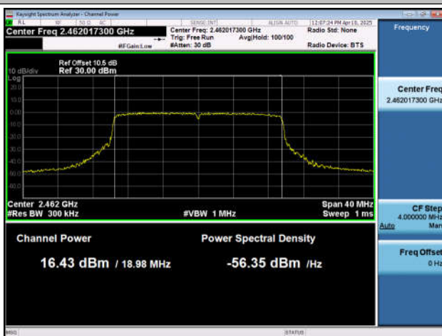
11BE20SISO-Ant4-2462-PASS
