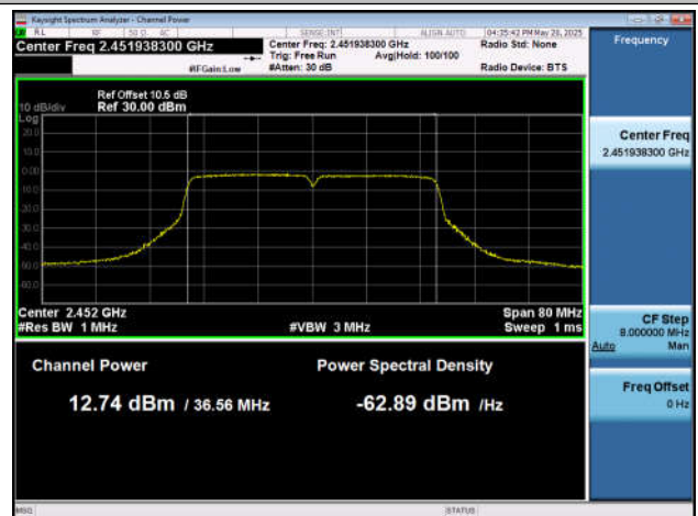
11N40MIMO-Ant7-2452-PASS
