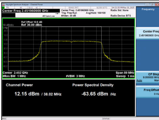
11BE40MIMO-Ant4-2452-PASS
