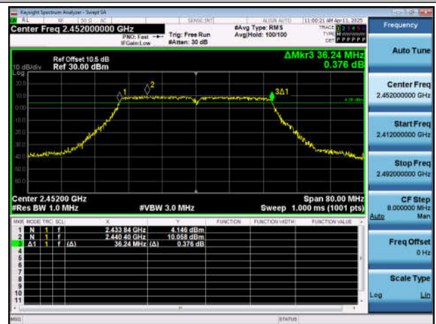
11N40SISO-Ant7-2452-PASS
