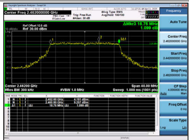
11AX20SISO-Ant7-2462-PASS
