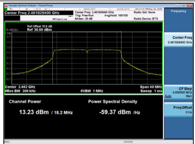
11N20MIMO-Ant7-2462-PASS
