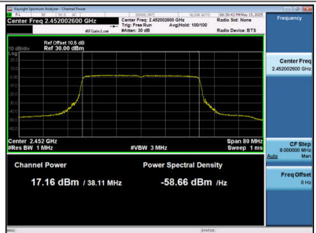
11BE40SISO-Ant7-2452-PASS
