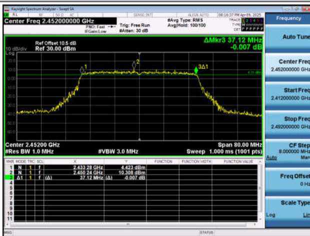
11AX40SISO-Ant4-2452-PASS
