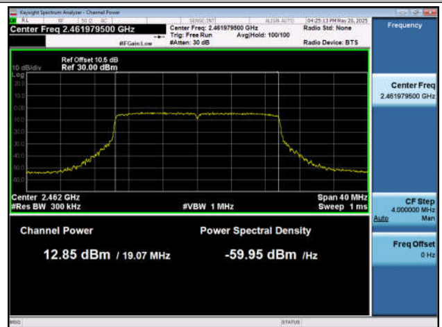
11AX20MIMO-Ant7-2462-PASS
