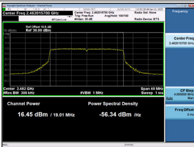
11AX20SISO-Ant4-2462-PASS
