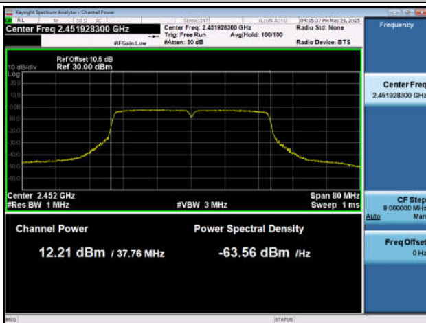
11N40MIMO-Ant4-2452-PASS
