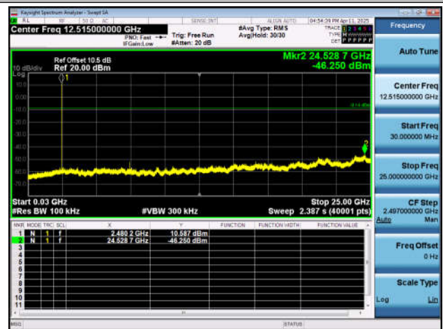
BLE_1M-Ant7-2480-30~25000-PASS
