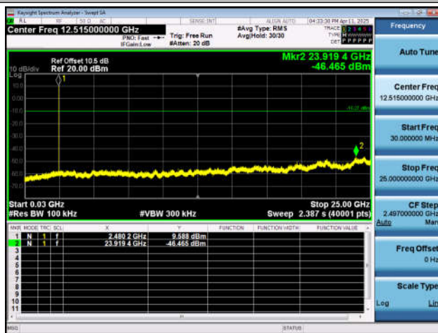
BLE_1M-Ant4-2480-30~25000-PASS
