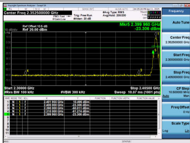
BLE_2M-Ant4-2402-PASS
