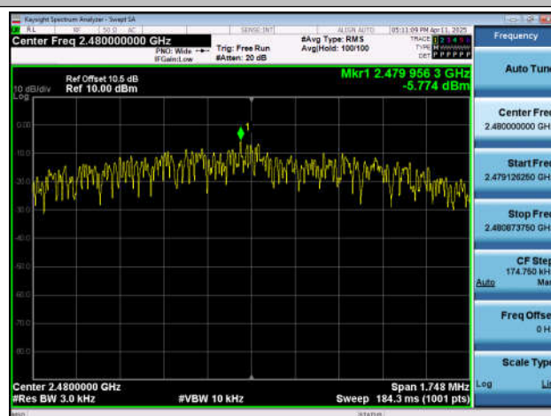
BLE_2M-Ant7-2480-PASS
