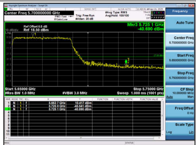
11BE40SISO-Ant6-5670-PASS
