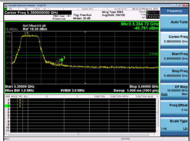
11AX20SISO-Ant6-5320-PASS
