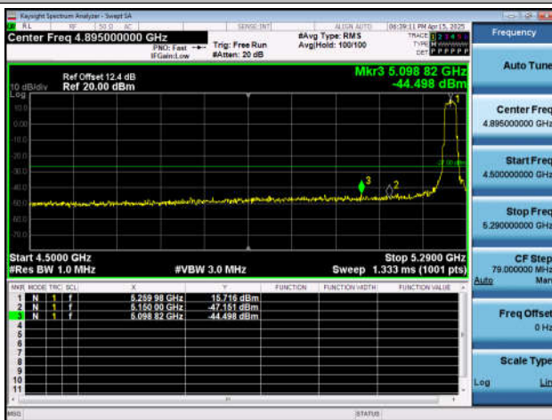
11BE20SISO-Ant4-5260-PASS
