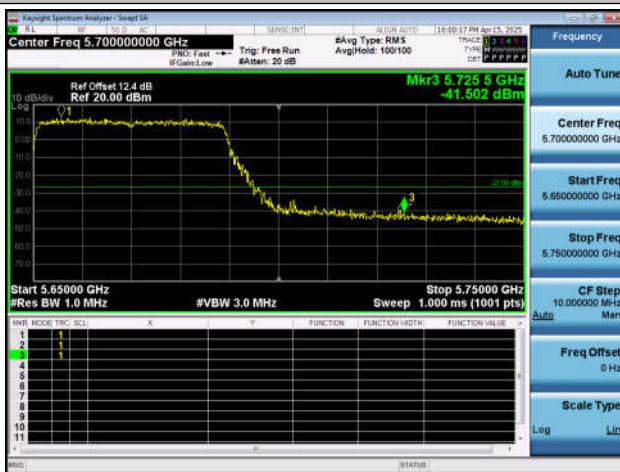
11BE40SISO-Ant4-5670-PASS
