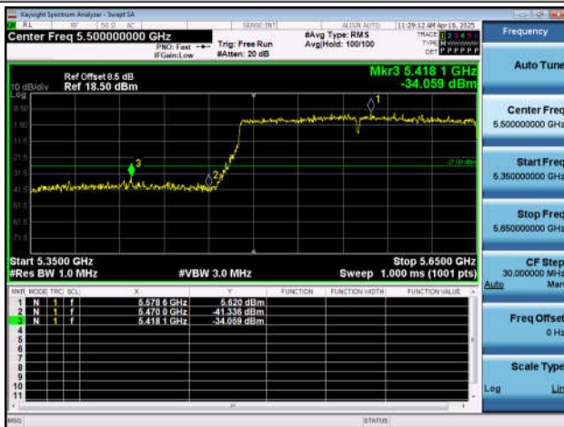
11AX160SISO-Ant6-5570-PASS
