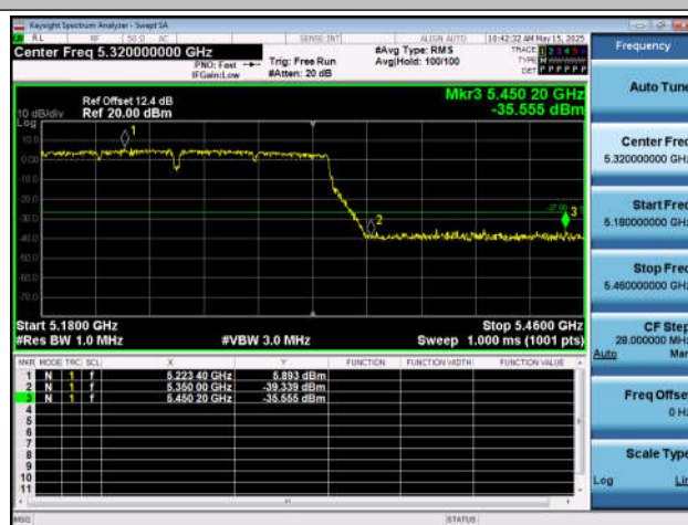
11AC160SISO-Ant6-5250-PASS
