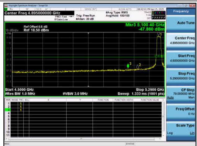
11BE20SISO-Ant6-5260-PASS
