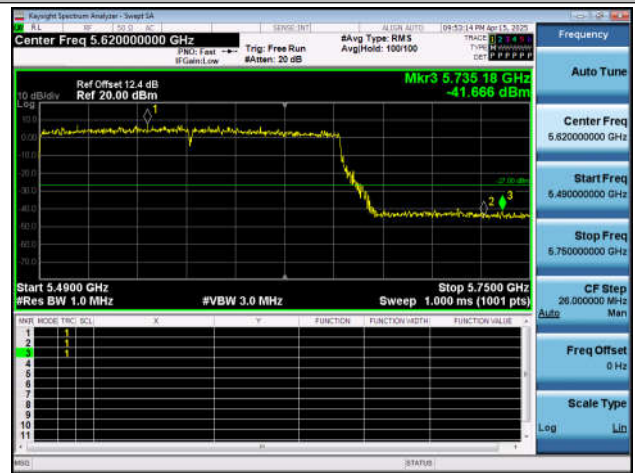
11AX160SISO-Ant6-5570-PASS
