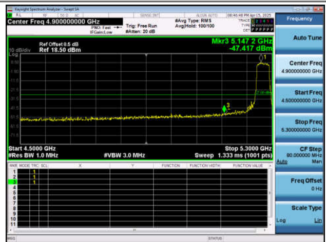
11BE40SISO-Ant6-5270-PASS
