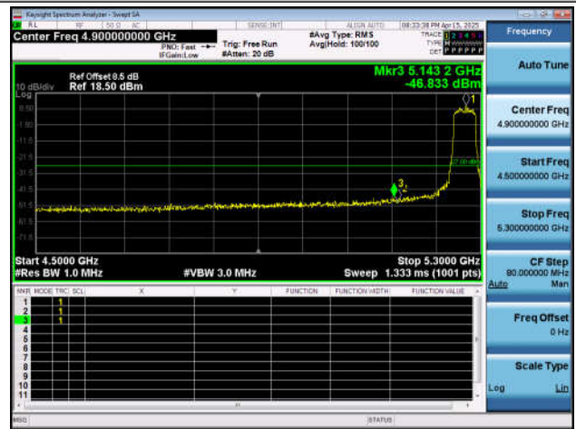
11AX40SISO-Ant6-5310-PASS
