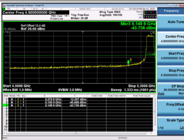
11BE40SISO-Ant4-5270-PASS
