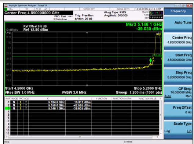
11AX20SISO-Ant6-5180-PASS
