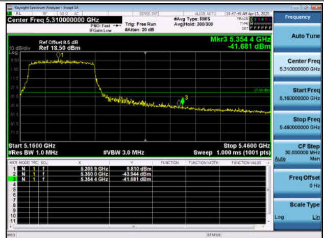
11AX80SISO-Ant4-5290-PASS
