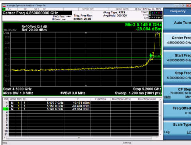
11AX20SISO-Ant4-5180-PASS
