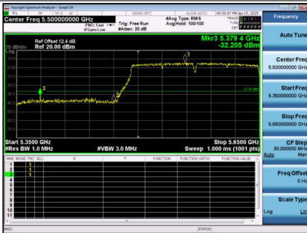
11AC160SISO-Ant6-5570-PASS
