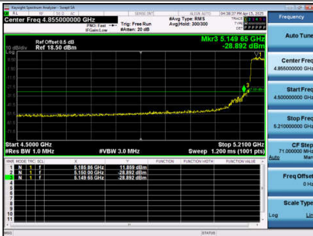
11BE40SISO-Ant4-5230-PASS
