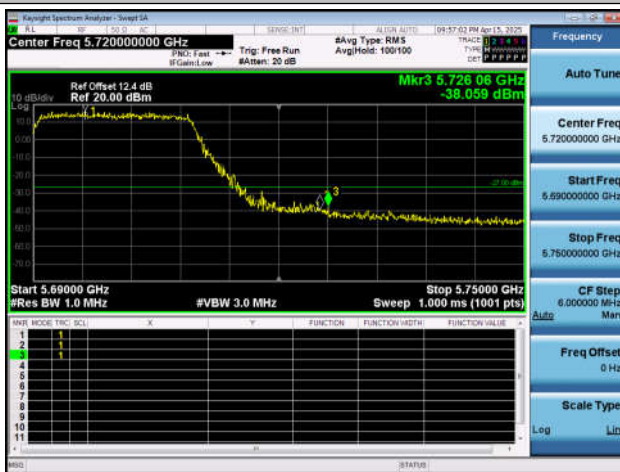
11BE20SISO-Ant4-5700-PASS
