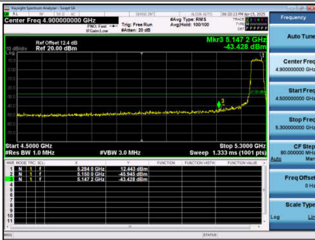
11AX40SISO-Ant4-5310-PASS
