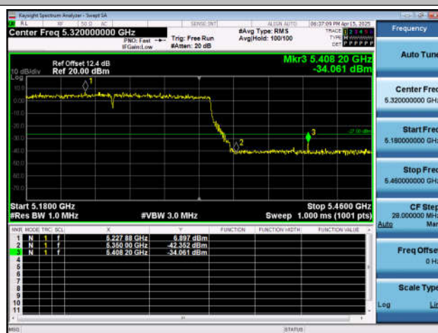
11AX160SISO-Ant4-5250-PASS
