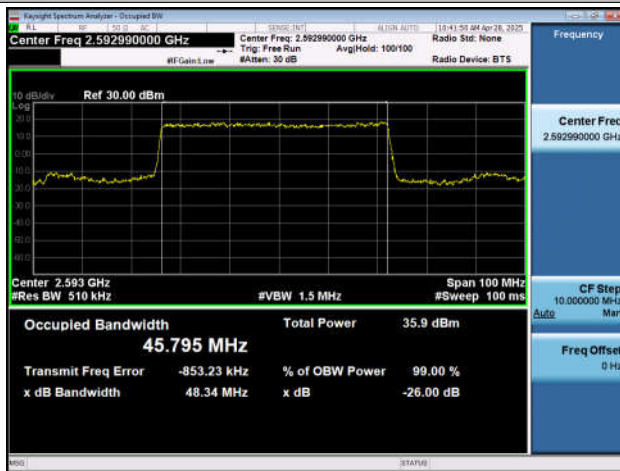
NTNV-n41-PC2-30-50-M-DFT-16QAM-Outer_Full-Ant1-PASS SS
