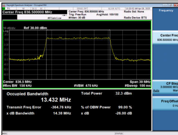
NTNV-n26(824-849)-PC3-15-20-M-DFT-QPSK-Outer_Full-A Ant1-PASS
