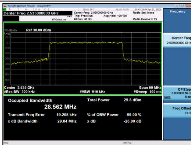
NTNV-n7-PC3-15-30-M-DFT-16QAM-Outer_Full-Ant1-PASS
