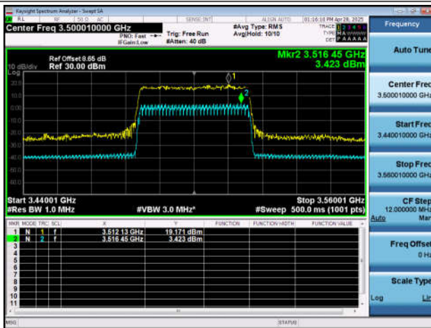
NTNT-n78(3450-3550)-PC2-30-50-M-CP-256QAM-Outer_ Full-Ant1-PASS
