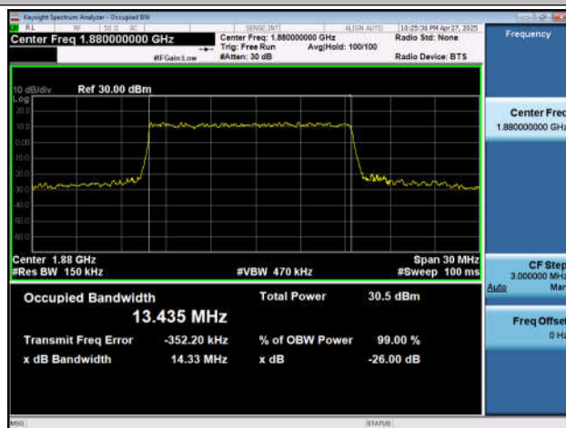
NTNV-n2-PC3-15-15-M-DFT-16QAM-Outter_Full-Ant1-PASS
