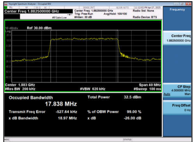
NTNV-n25-PC3-15-20-M-DFT-16QAM-Outer_Full-Ant1-PASS SS
