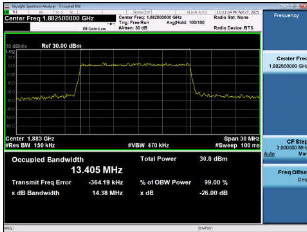
NTNV-n25-PC3-15-20-M-DFT-QPSK-Outer_Full-Ant1-PASS S
