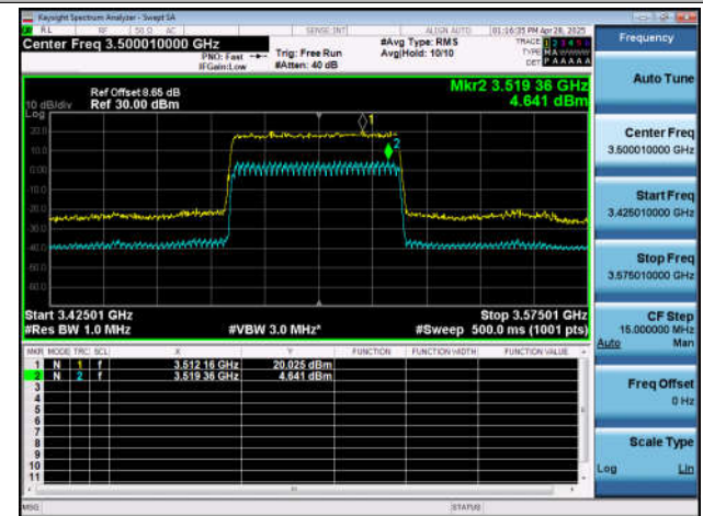
NTNT-n78(3450-3550)-PC2-30-60-M-DFT-256QAM-Outer_ Full-Ant1-PASS
