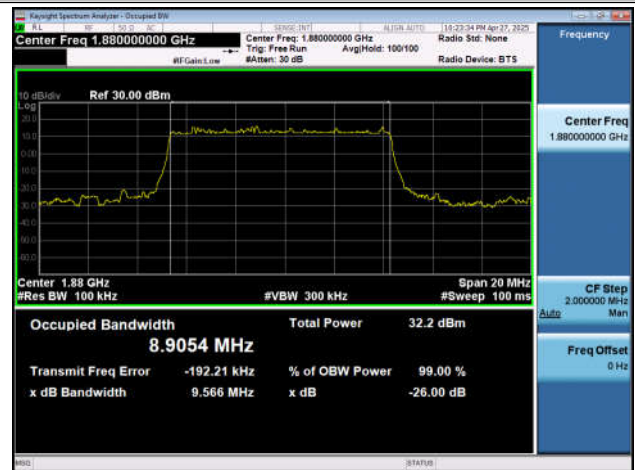
NTNV-n2-PC3-15-10-M-DFT-16QAM-Outer_Full-Ant1-PASS
