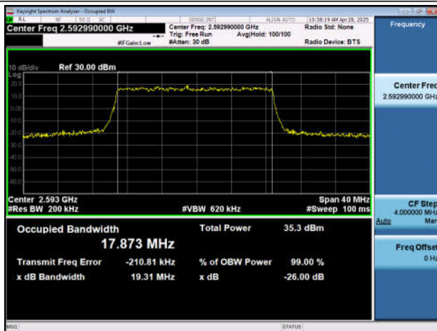
NTNV-n41-PC2-30-20-M-DFT-QPSK-Outer_Full-Ant1-PASS
