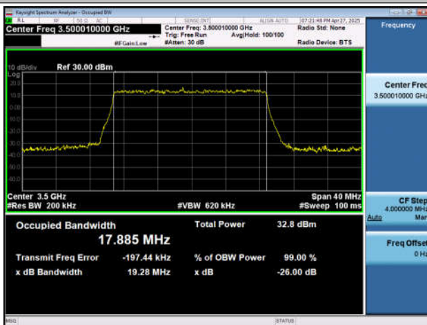
NTNV-n77(3450-3550)-PC2-30-20-M-DFT-QPSK-Outet_Ful
