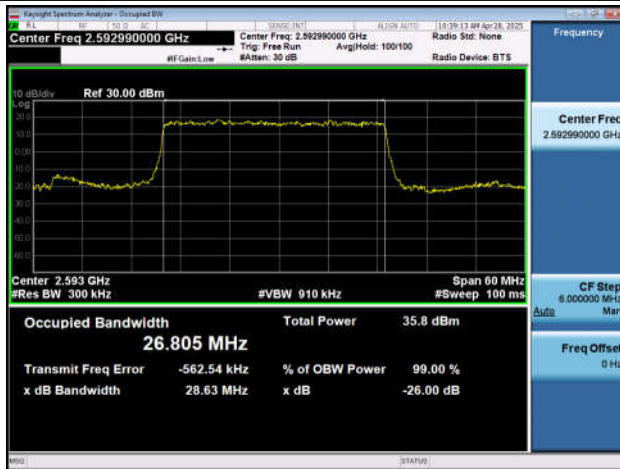
NTNV-n41-PC2-30-30-M-DFT-16QAM-Outer_Full-Ant1-PASS SS
