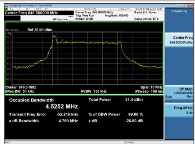
NTNV-n5-PC3-15-5-H-DFT-16QAM-Outer_Full-Ant1-PASS
