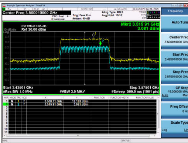
NTNT-n78(3450-3550)-PC2-30-60-M-CP-256QAM-Outer_ Full-Ant1-PASS
