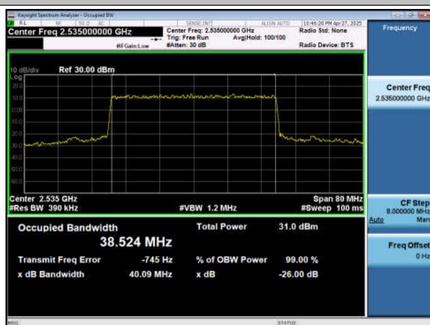
NTNV-n7-PC3-15-40-M-DFT-QPSK-Outer_Full-Ant1-PASS
