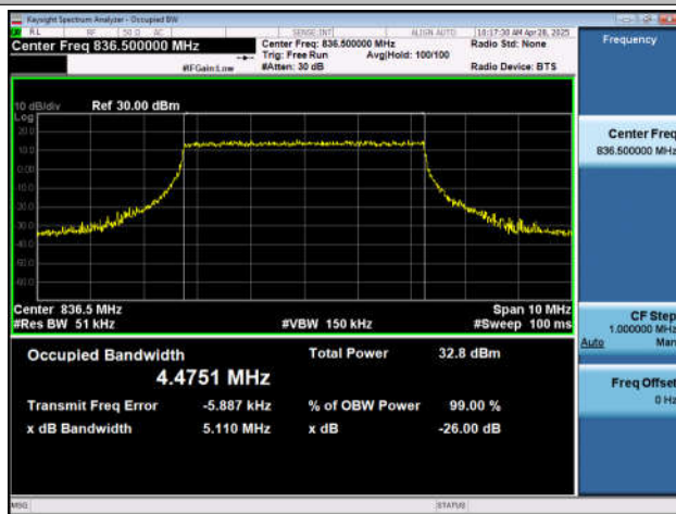
NTNV-n26(824-849)-PC3-15-10-M-DFT-QPSK-Outer_Full- Ant1-PASS
