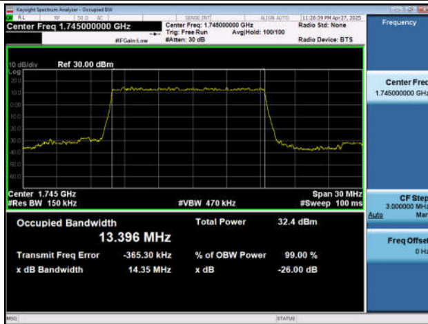
NTNV-n66-PC3-15-15-M-DFT-16QAM-Outer_Full-Ant1-PASS
