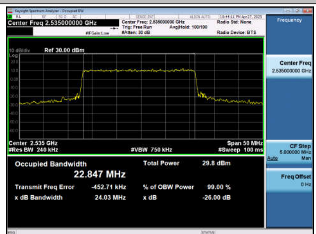
NTNV-n7-PC3-15-25-M-DFT-16QAM-Outer_Full-Ant1-PASS
