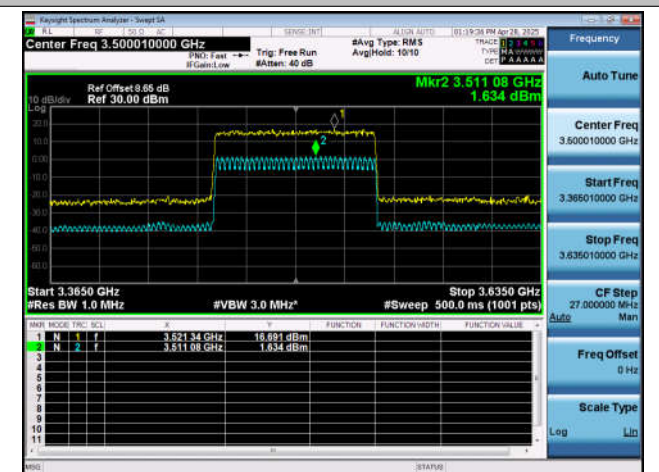
NTNT-n78(3450-3550)-PC2-30-100-M-DFT-256QAM-Outer_Full-Ant1-PASS
