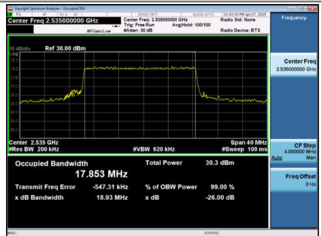
NTNV-n7-PC3-15-20-M-DFT-QPSK-Outer_Full-Ant1-PASS
