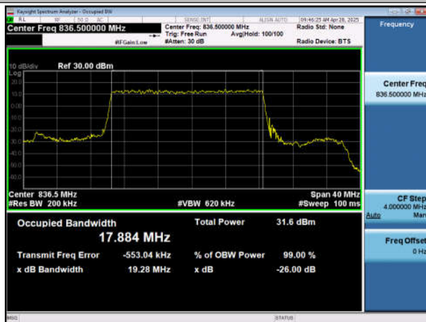
NTNV-n5-PC3-15-20-M-DFT-16QAM-Outet_Full-Ant1-PASS
