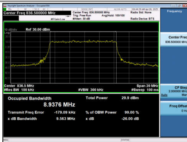
NTNV-n5-PC3-15-10-M-DFT-16QAM-Outter_Full-Ant1-PASS
