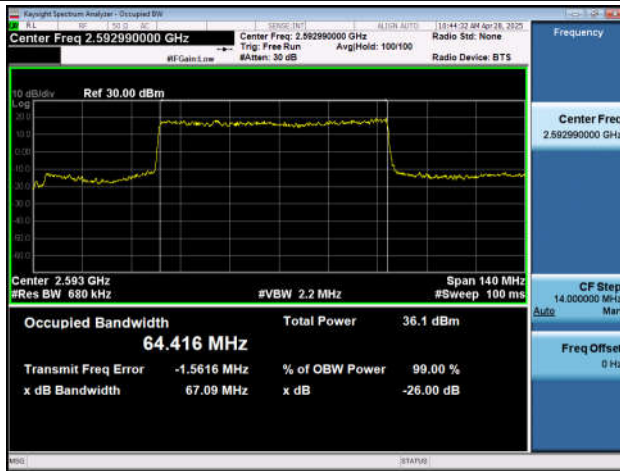
NTNV-n41-PC2-30-70-M-DFT-16QAM-Outer_Full-Ant1-PASS SS
