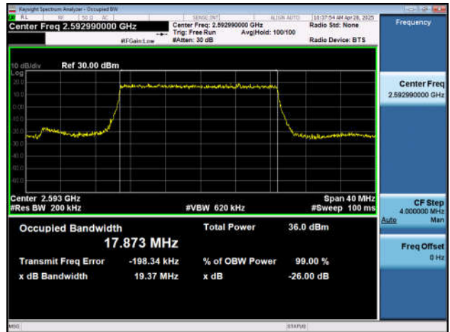
NTNV-n41-PC2-30-20-M-DFT-16QAM-Outer_Full-Ant1-PASS
