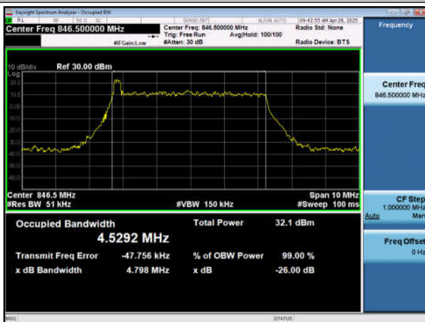
NTNV-n5-PC3-15-5-H-DFT-QPSK-Outer_Full-Ant1-PASS
