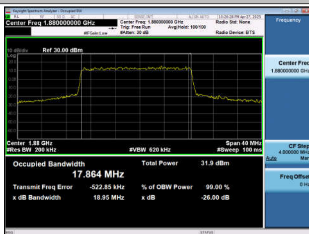
NTNV-n2-PC3-15-20-M-DFT-QPSK-Outter_Full-Ant1-PASS
