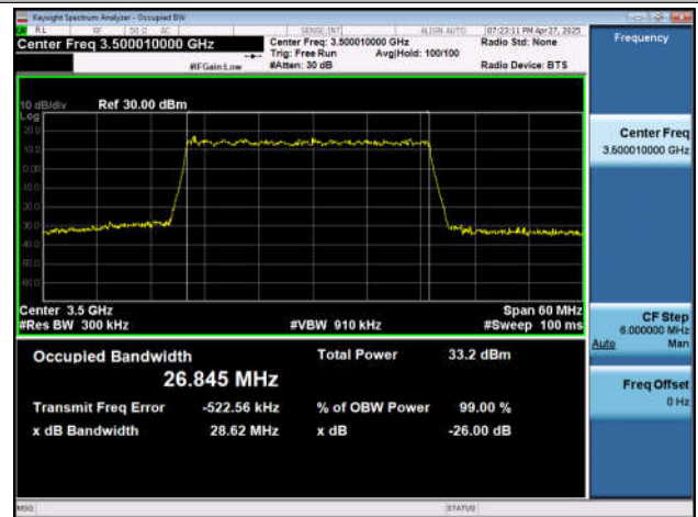
NTNV-n77(3450-3550)-PC2-30-40-M-DFT-BPSK-Outet_Ful
