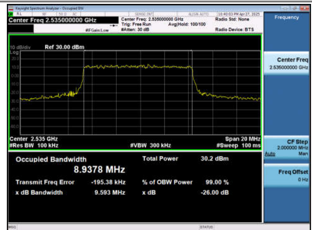
NTNV-n7-PC3-15-10-M-DFT-QPSK-Outter_Full-Ant1-PASS
