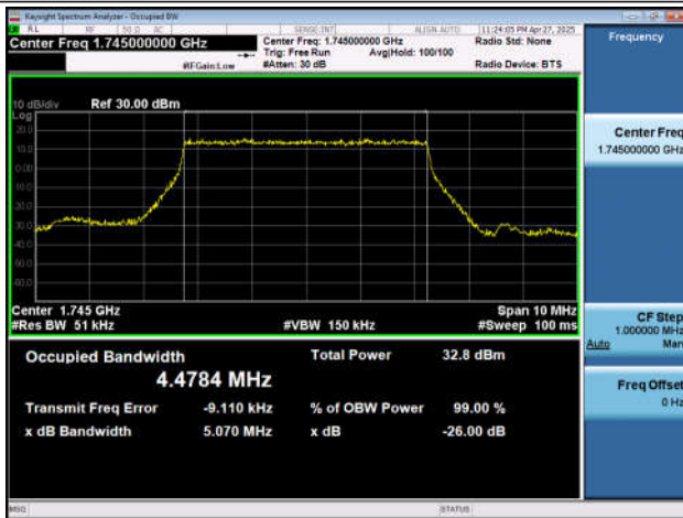
NTNV-n66-PC3-15-5-M-DFT-16QAM-Outet_Full-Ant1-PAS
