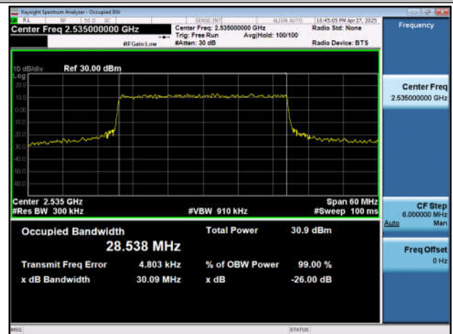
NTNV-n7-PC3-15-30-M-DFT-QPSK-Outer_Full-Ant1-PASS
