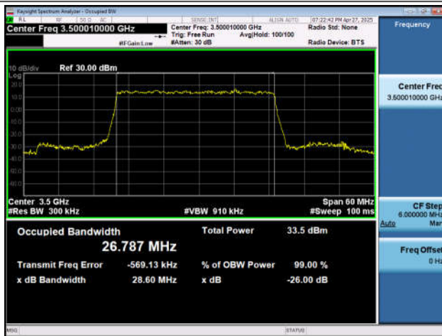
NTNV-n77(3450-3550)-PC2-30-30-M-DFT-16QAM-Outet_F
