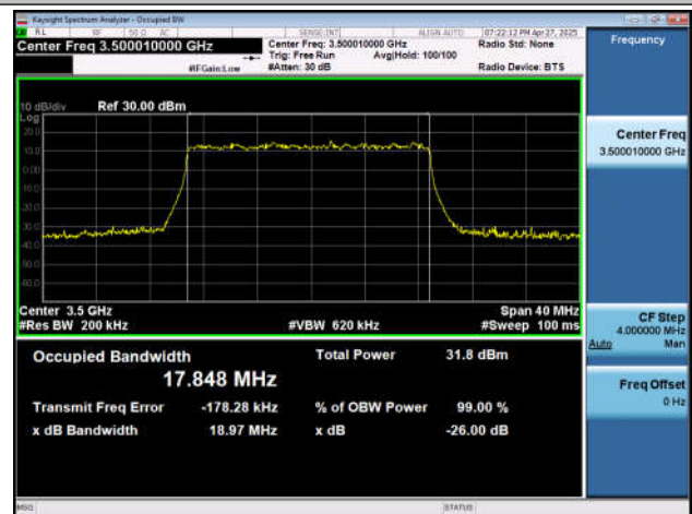
NTNV-n77(3450-3550)-PC2-30-20-M-DFT-16QAM-Outet_F
