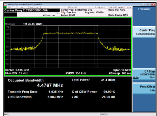
NTNV-n7-PC3-15-5-M-DFT-16QAM-Outet_Full-Ant1-PASS
