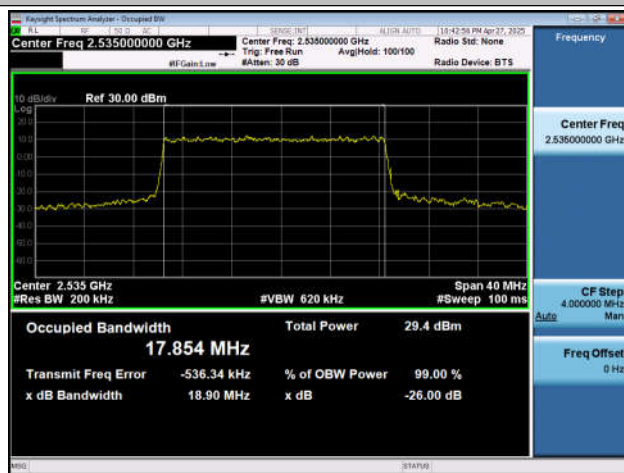
NTNV-n7-PC3-15-20-M-DFT-16QAM-Outer_Full-Ant1-PASS
