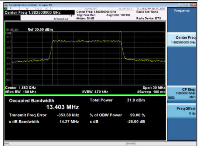
NTNV-n25-PC3-15-15-M-DFT-QPSK-Outer_Full-Ant1-PASS S
