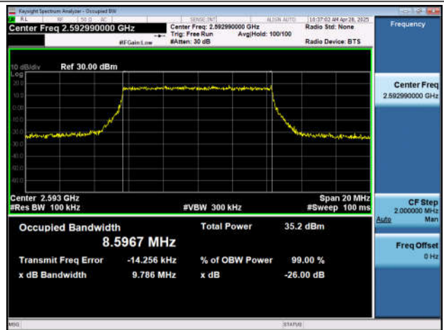
NTNV-n41-PC2-30-10-M-DFT-QPSK-Outer_Full-Ant1-PASS
