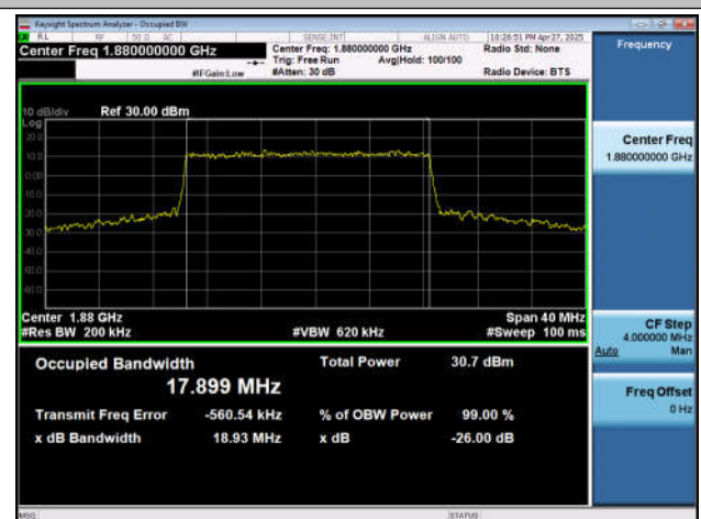
NTNV-n2-PC3-15-20-M-DFT-16QAM-Outter_Full-Ant1-PASS
