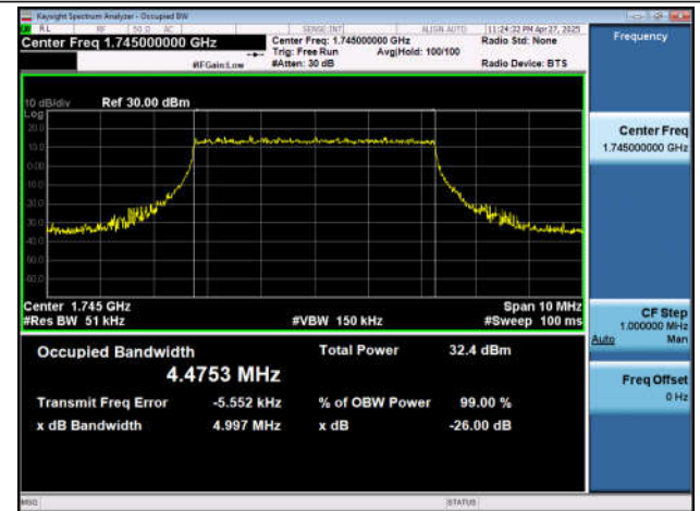
NTNV-n66-PC3-15-5-M-DFT-QPSK-Outet_Full-Ant1-PASS
