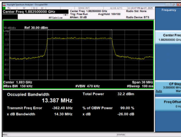
NTNV-n25-PC3-15-15-M-DFT-16QAM-Outer_Full-Ant1-PASS SS
