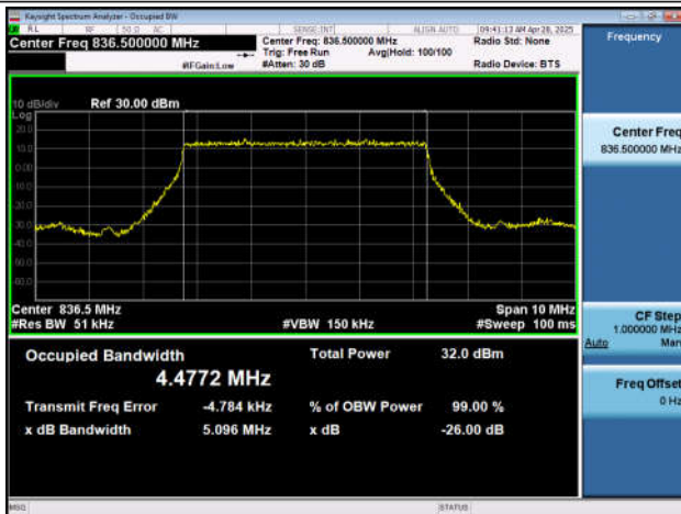
NTNV-n5-PC3-15-5-M-DFT-16QAM-Outer_Full-Ant1-PASS
