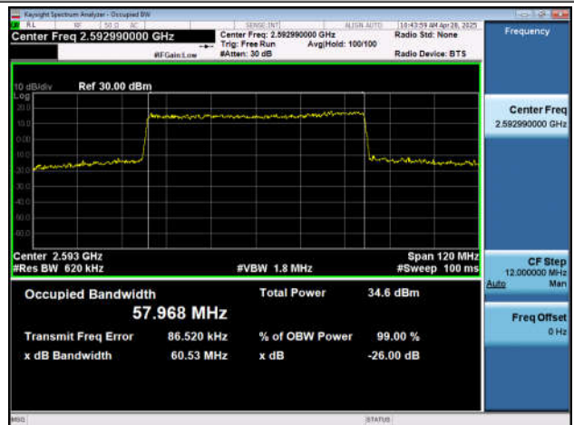
NTNV-n41-PC2-30-60-M-DFT-16QAM-Outer_Full-Ant1-PASS SS
