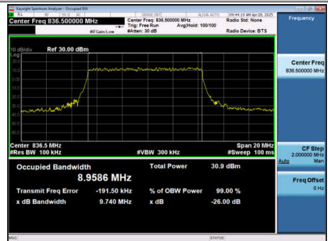
NTNV-n5-PC3-15-10-M-DFT-QPSK-Outter_Full-Ant1-PASS
