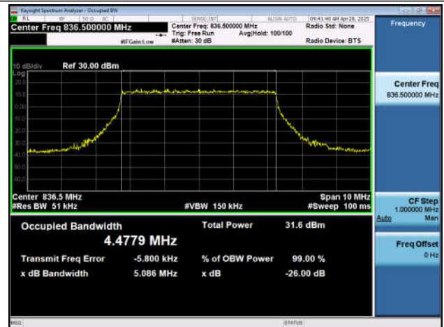
NTNV-n5-PC3-15-5-H-DFT-BPSK-Outer_Full-Ant1-PASS
