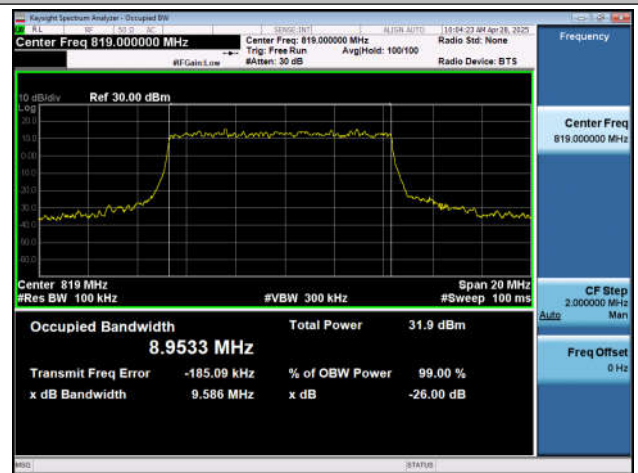
NTNV-n26(814-824)-PC3-15-10-M-DFT-16QAM-Outer_Full- Ant1-PASS
