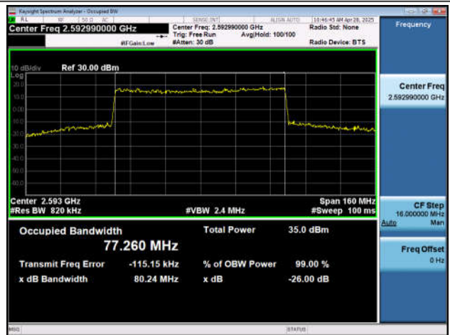
NTNV-n41-PC2-30-80-M-DFT-16QAM-Outer_Full-Ant1-PASS SS
