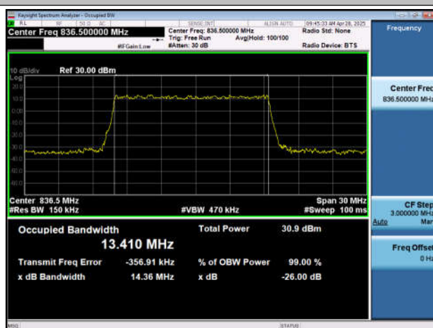
NTNV-n5-PC3-15-15-M-DFT-QPSK-Outter_Full-Ant1-PASS
