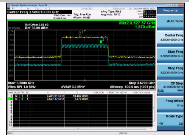
NTNT-n78(3450-3550)-PC2-30-90-M-DFT-256QAM-Outter_F ull-Ant1-PASS
