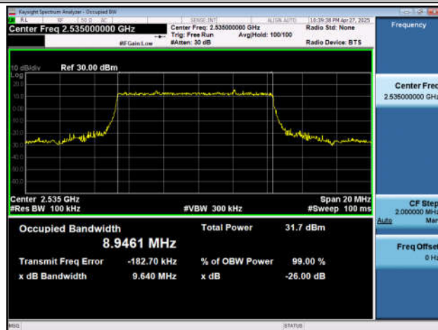
NTNV-n7-PC3-15-10-M-DFT-16QAM-Outter_Full-Ant1-PASS
