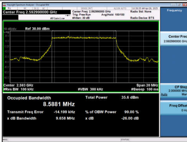
NTNV-n41-PC2-30-10-M-DFT-16QAM-Outer_Full-Ant1-PASS
