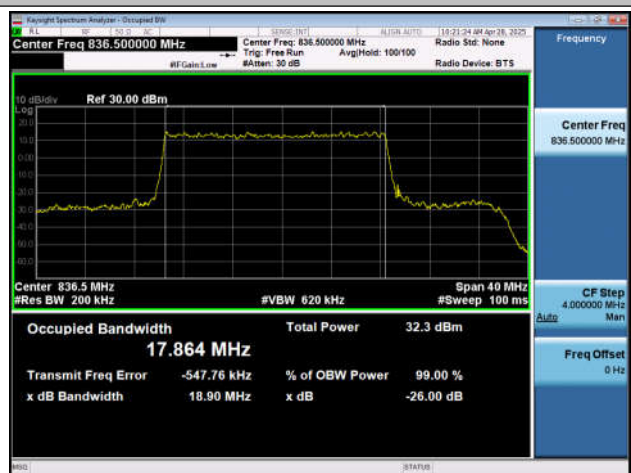
NTNV-n26(824-849)-PC3-15-20-M-DFT-16QAM-Outer_Full -Ant1-PASS
