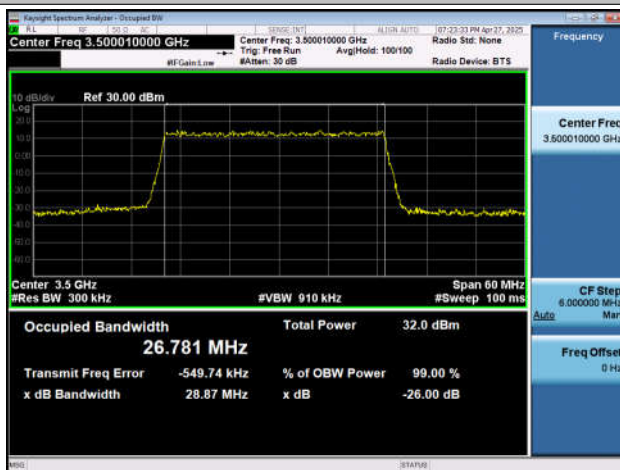
NTNV-n77(3450-3550)-PC2-30-40-M-DFT-QPSK-Outet_Ful
