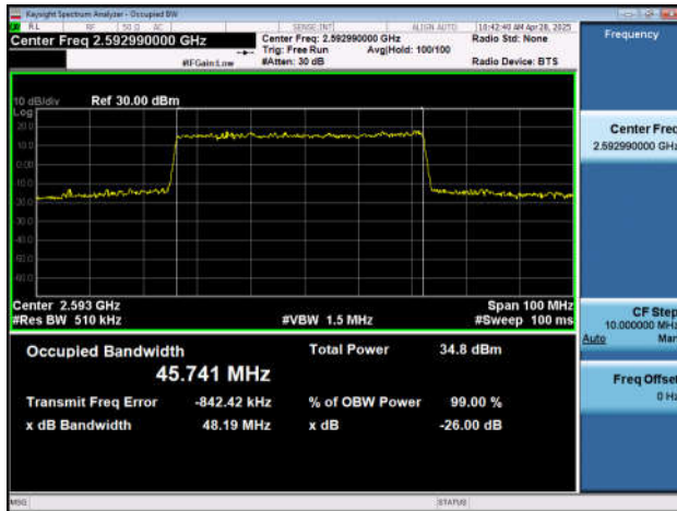
NTNV-n41-PC2-30-60-M-DFT-QPSK-Outer_Full-Ant1-PASS S
