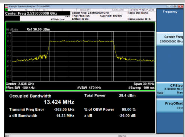
NTNV-n7-PC3-15-15-M-DFT-16QAM-Outter_Full-Ant1-PASS
