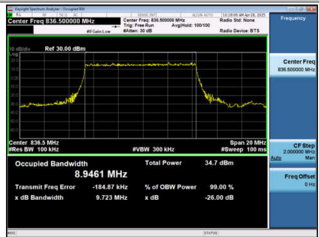
NTNV-n26(824-849)-PC3-15-10-M-DFT-16QAM-Outer_Full- Ant1-PASS
