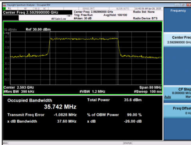
NTNV-n41-PC2-30-40-M-DFT-QPSK-Outer_Full-Ant1-PASS S
