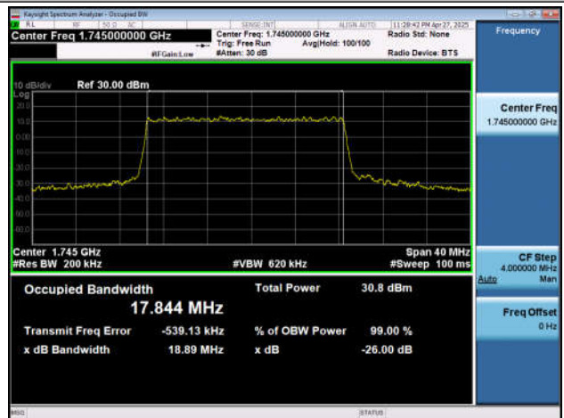
NTNV-n66-PC3-15-20-M-DFT-16QAM-Outer_Full-Ant1-PASS
