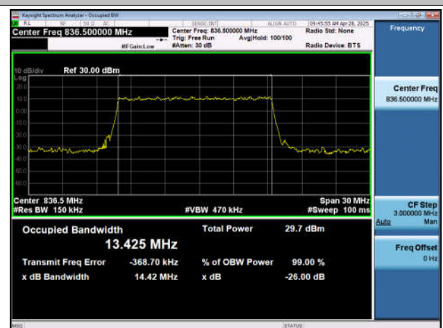
NTNV-n5-PC3-15-15-M-DFT-16QAM-Outter_Full-Ant1-PASS
