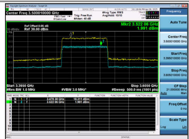
NTNT-n78(3450-3550)-PC2-30-70-M-DFT-256QAM-Outer_ Full-Ant1-PASS
