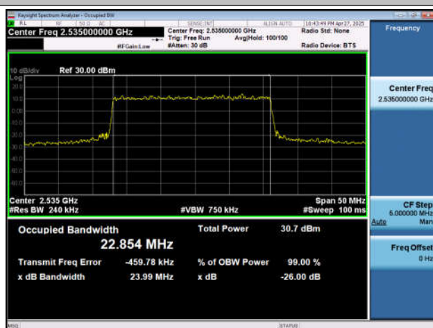
NTNV-n7-PC3-15-25-M-DFT-QPSK-Outer_Full-Ant1-PASS
