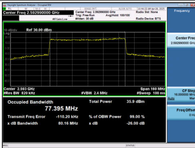
NTNV-n41-PC2-30-80-M-DFT-QPSK-Outer_Full-Ant1-PASS S
