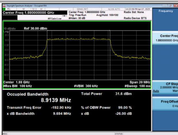
NTNV-n2-PC3-15-10-M-DFT-QPSK-Outer_Full-Ant1-PASS
