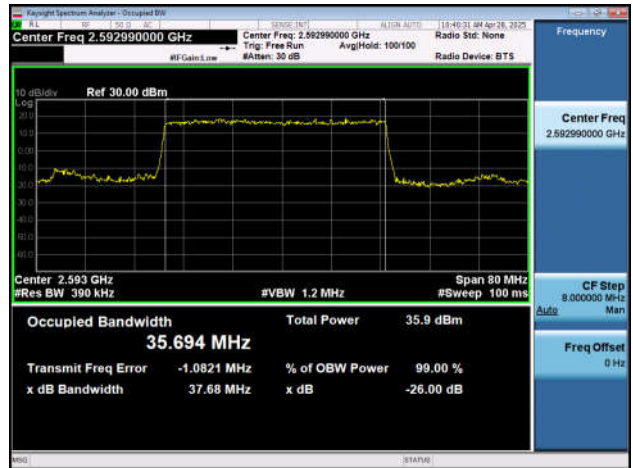
NTNV-n41-PC2-30-40-M-DFT-16QAM-Outer_Full-Ant1-PASS SS
