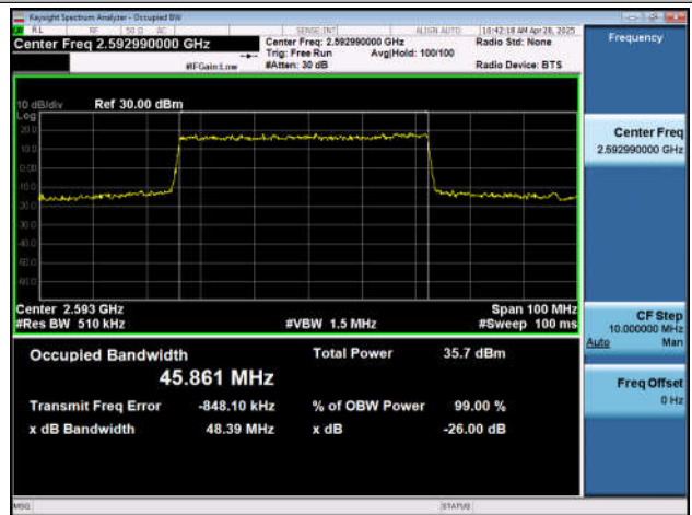
NTNV-n41-PC2-30-50-M-DFT-QPSK-Outer_Full-Ant1-PASS S
