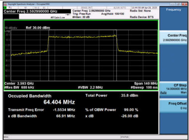
NTNV-n41-PC2-30-70-M-DFT-QPSK-Outer_Full-Ant1-PASS S
