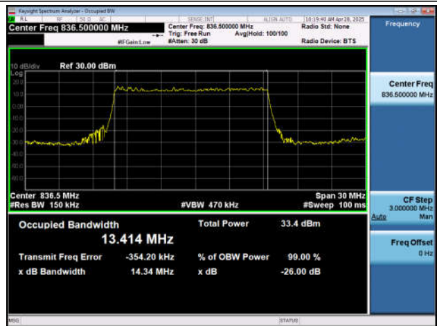
NTNV-n26(824-849)-PC3-15-20-M-DFT-BPSK-Outer_Full-A nt1-PASS
