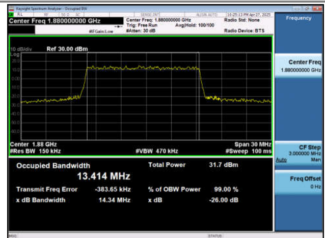
NTNV-n2-PC3-15-15-M-DFT-QPSK-Outter_Full-Ant1-PASS
