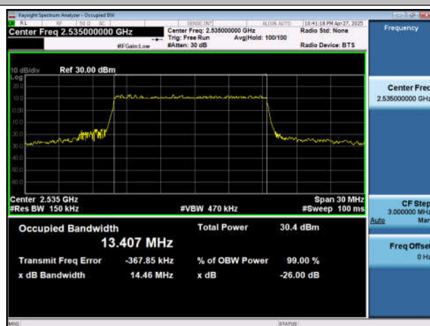
NTNV-n7-PC3-15-15-M-DFT-QPSK-Outter_Full-Ant1-PASS
