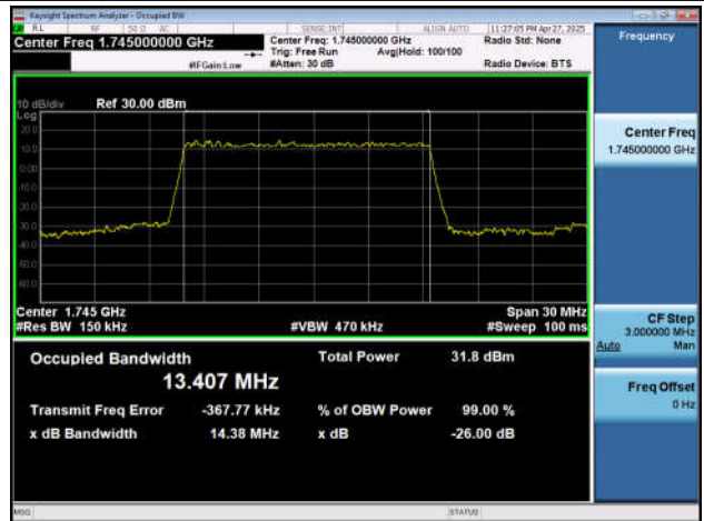
NTNV-n66-PC3-15-15-M-DFT-QPSK-Outer_Full-Ant1-PASS
