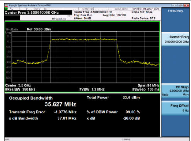
NTNV-n77(3450-3550)-PC2-30-40-M-DFT-16QAM-Outet_F
