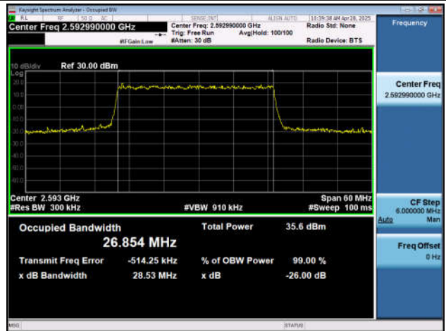
NTNV-n41-PC2-30-30-M-DFT-QPSK-Outer_Full-Ant1-PASS S
