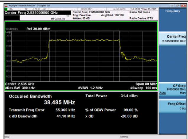
NTNV-n7-PC3-15-40-M-DFT-16QAM-Outer_Full-Ant1-PASS
