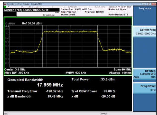
NTNV-n77(3450-3550)-PC2-30-20-M-DFT-16QAM-Outet_F
