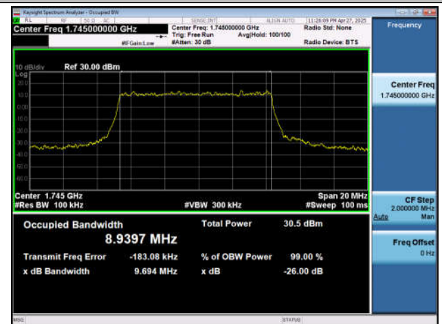
NTNV-n66-PC3-15-10-M-DFT-16QAM-Outet_Full-Ant1-PAS
