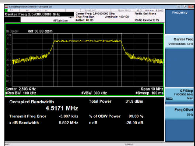
Band41-5MHz-16QAM-40620-25RB#0-PASS
