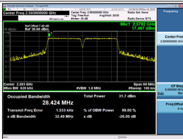
41-41-15MHz-15MHz-QPSK-QPSK-40545-40695-75RB#0 -75RB#0-PASS
