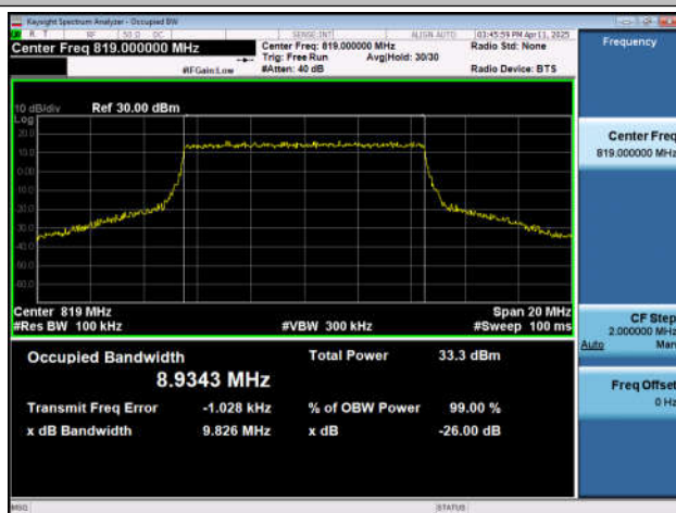
Band26(814-824)-10MHz-QPSK-26740-50RB#0-PASS
