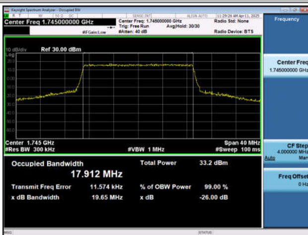
Band66-20MHz-QPSK-132322-100RB#0-PASS
