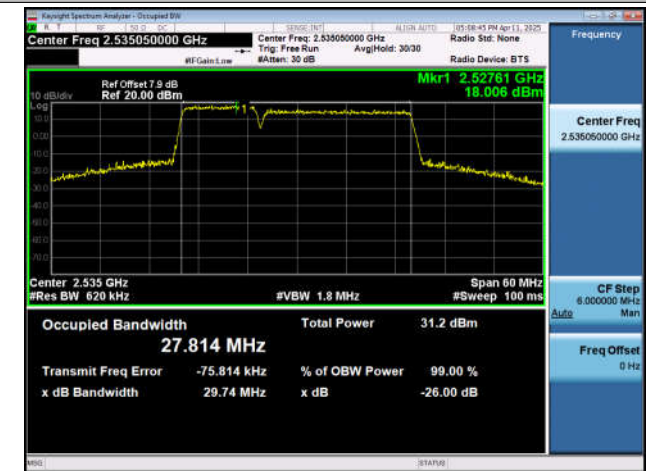
7-7-15MHz-10MHz-16QAM-16QAM-21051-21171-75RB#0-5 0RB#0-PASS
