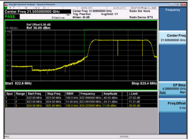
Band5-1.4MHz-QPSK-20643-6RB#0-PASS
