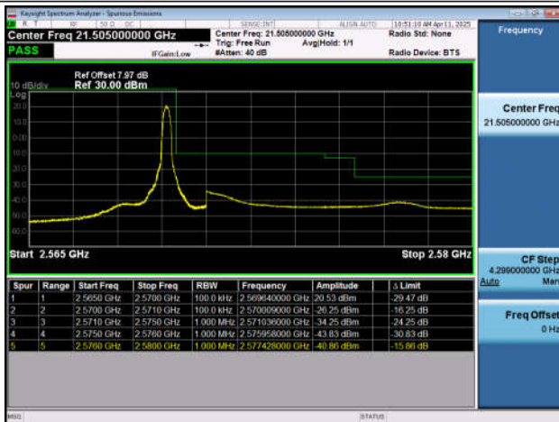
Band7-10MHz-QPSK-20800-1RB#0-PASS
