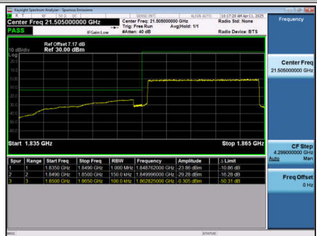
Band2-15MHz-QPSK-18675-75RB#0-PASS
