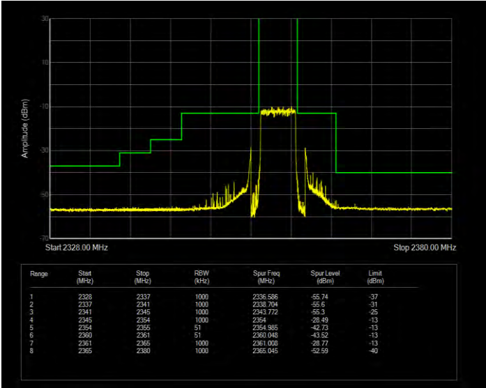
Band40(2350-2360) QPSK BW=5MHz Channel=39225 RB Size=1 Position=#0 Extended
