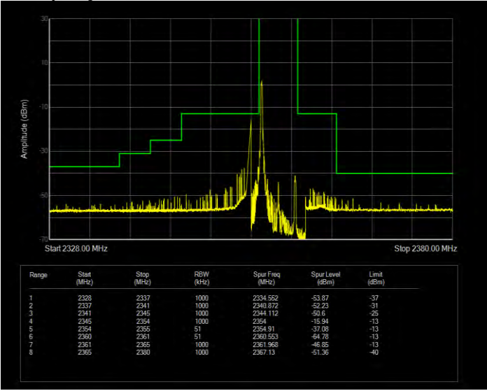
Band40(2350-2360) QPSK BW=10MHz Channel=39200 RB Size=50 Position=#0 Extended
