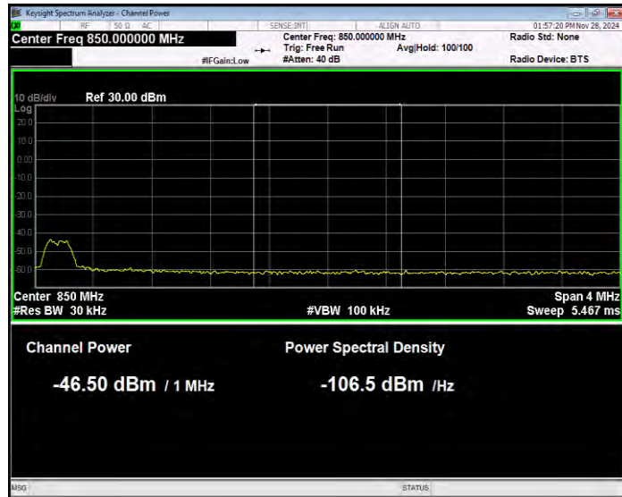
Band26(824-849) QPSK BW=15MHz Channel=26865 RB Size=75 Position=#0 Normal
