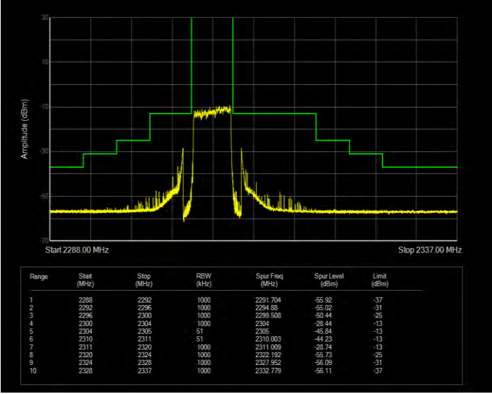
Band40(2305-2315) 16QAM BW=5MHz Channel=38775 RB Size=1 Position=#0 Extended
