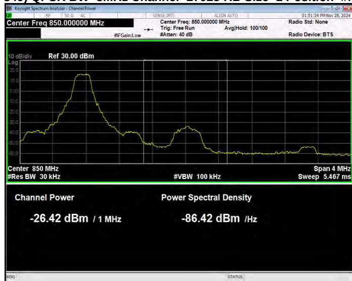
Band26(824-849) QPSK BW=3MHz Channel=27025 RB Size=1 Position=#Max Normal
