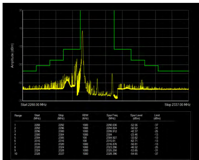
Band40(2305-2315) QPSK BW=10MHz Channel=38750 RB Size=50 Position=#0 Extended
