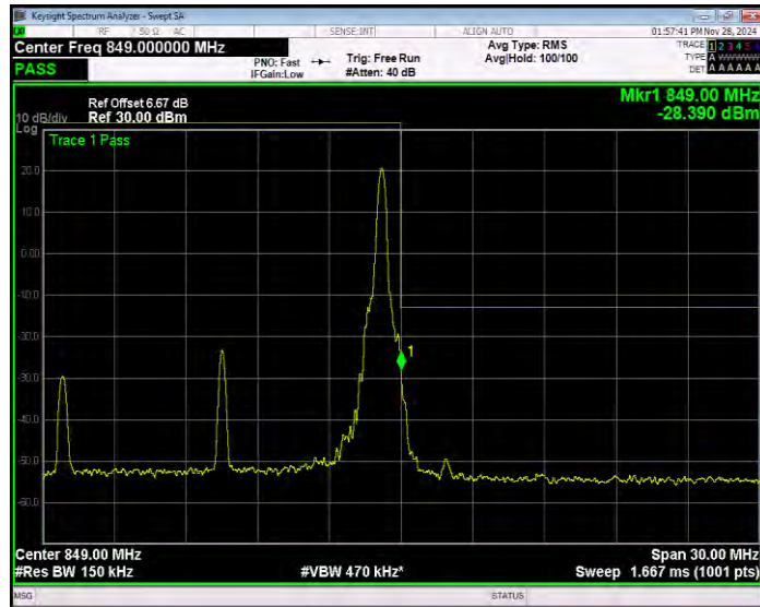
Band26(824-849) 16QAM BW=15MHz Channel=26965 RB Size=75 Position=#0 Extended
