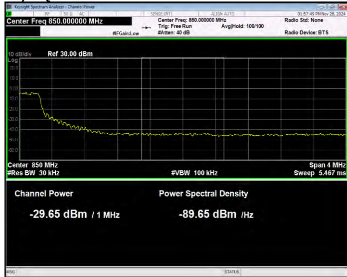
Band26(824-849) 16QAM BW=15MHz Channel=26965 RB Size=1 Position=#Max Extended
