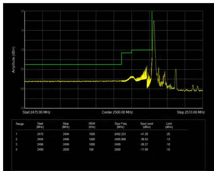
Band7 QPSK BW=5MHz Channel=20775 RB Size=1 Position=#Max Extended
