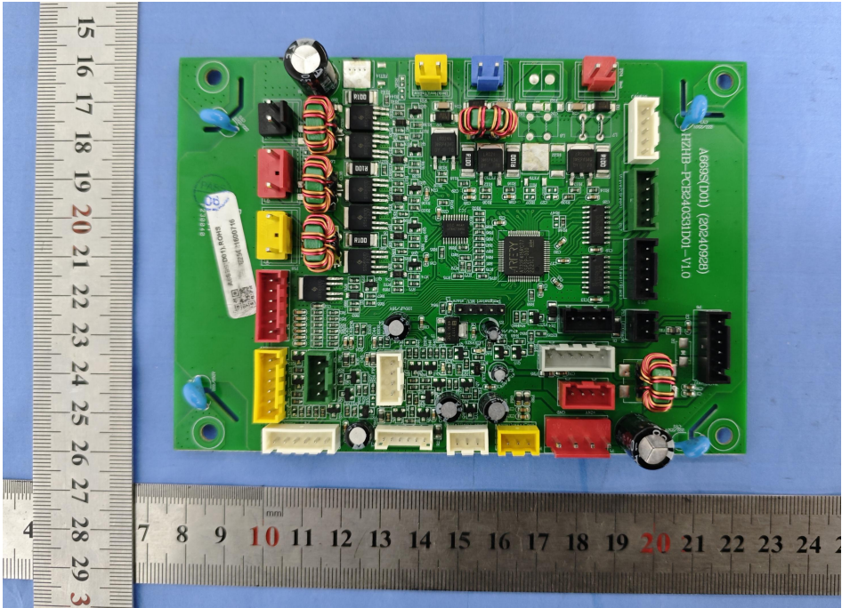
INTERNAL PHOTO OF SAMPLE PCB
