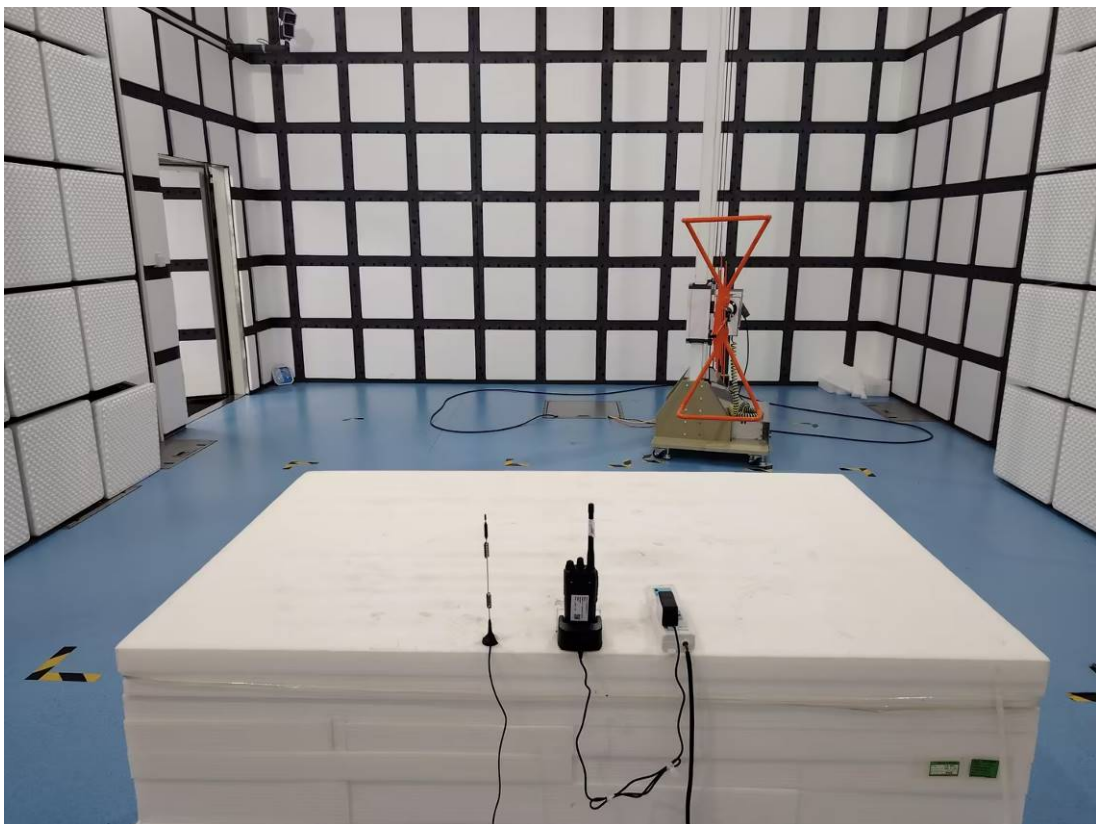
RE- 30MHz~1GHz Rear View(Mode 2)
