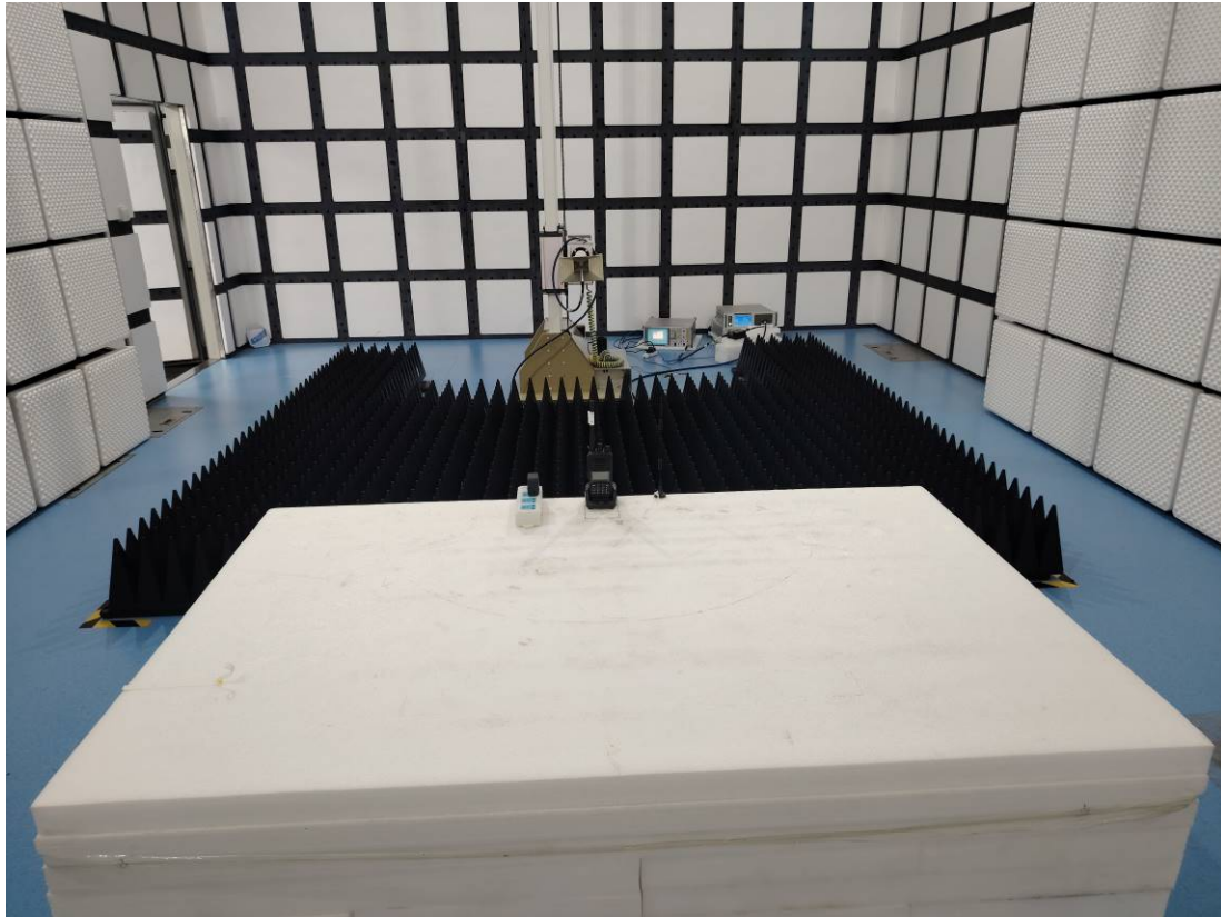
RE- 1GHz-5GHz Rear View (Mode 2)
