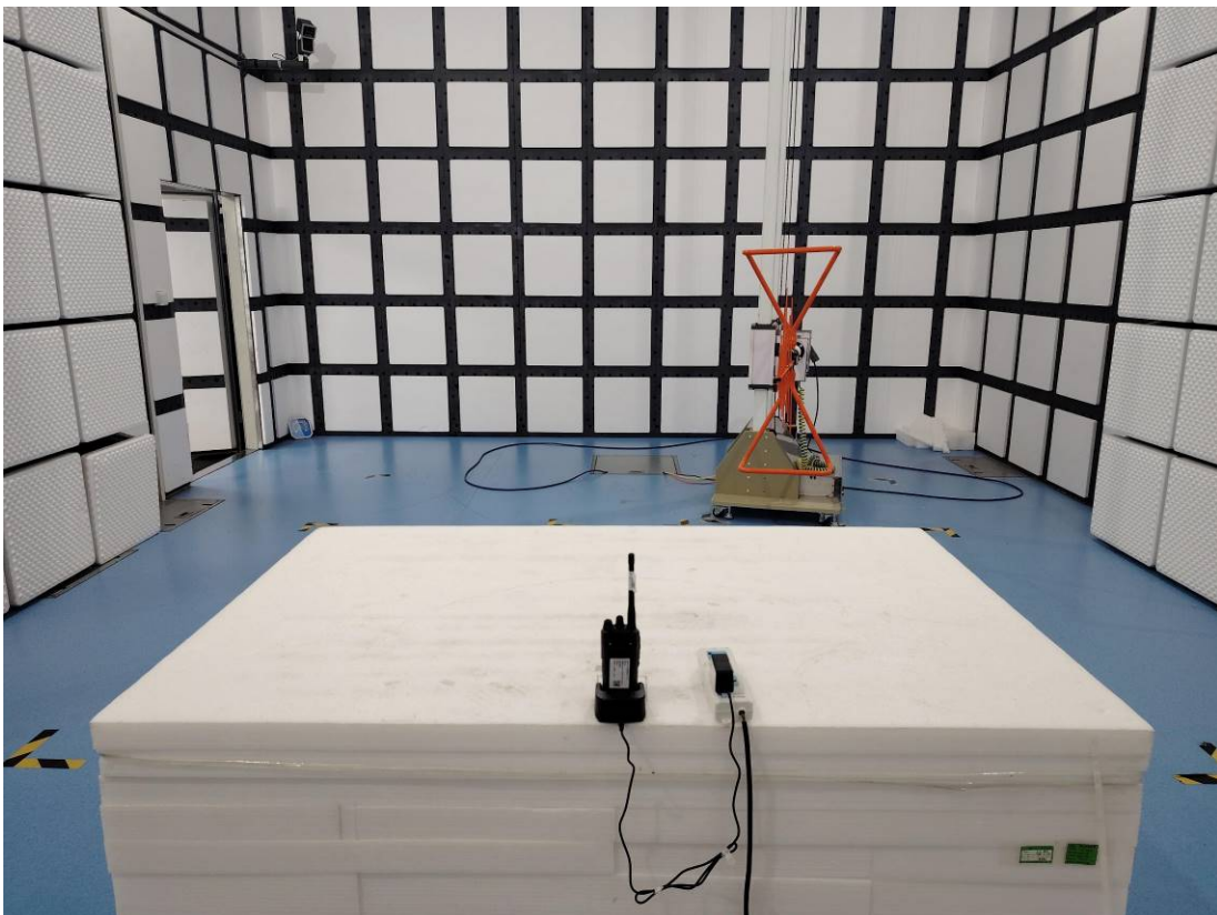
RE- 30MHz-1GHz Rear View(Mode 1)
