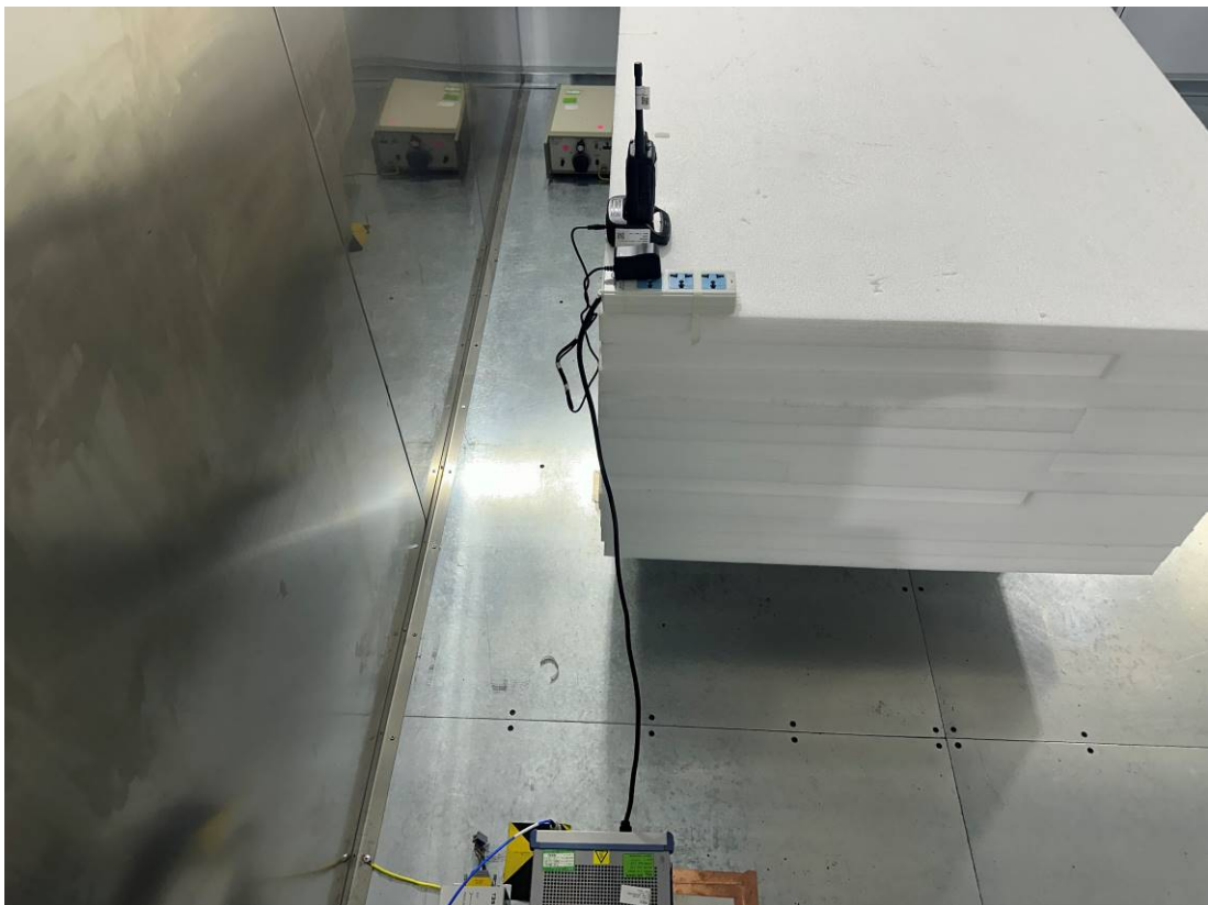
CE- Rear View (Mode 1)
