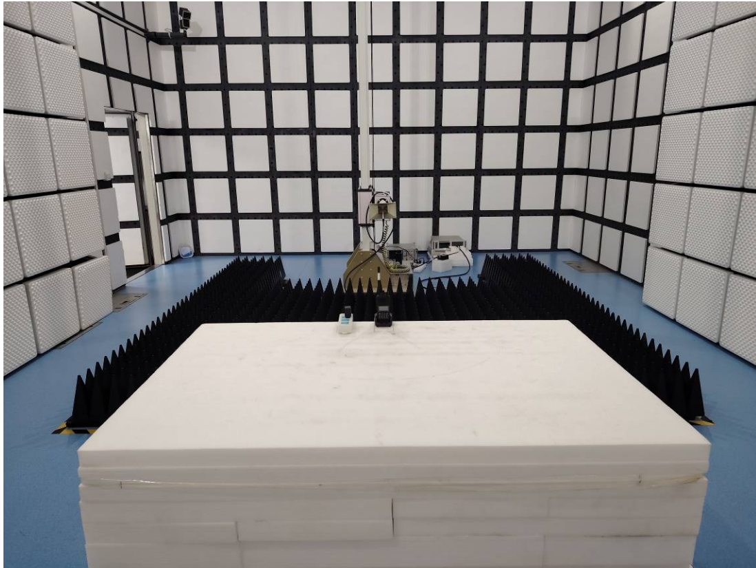
RE- 1GHz-5GHz Rear View (Mode 1)
