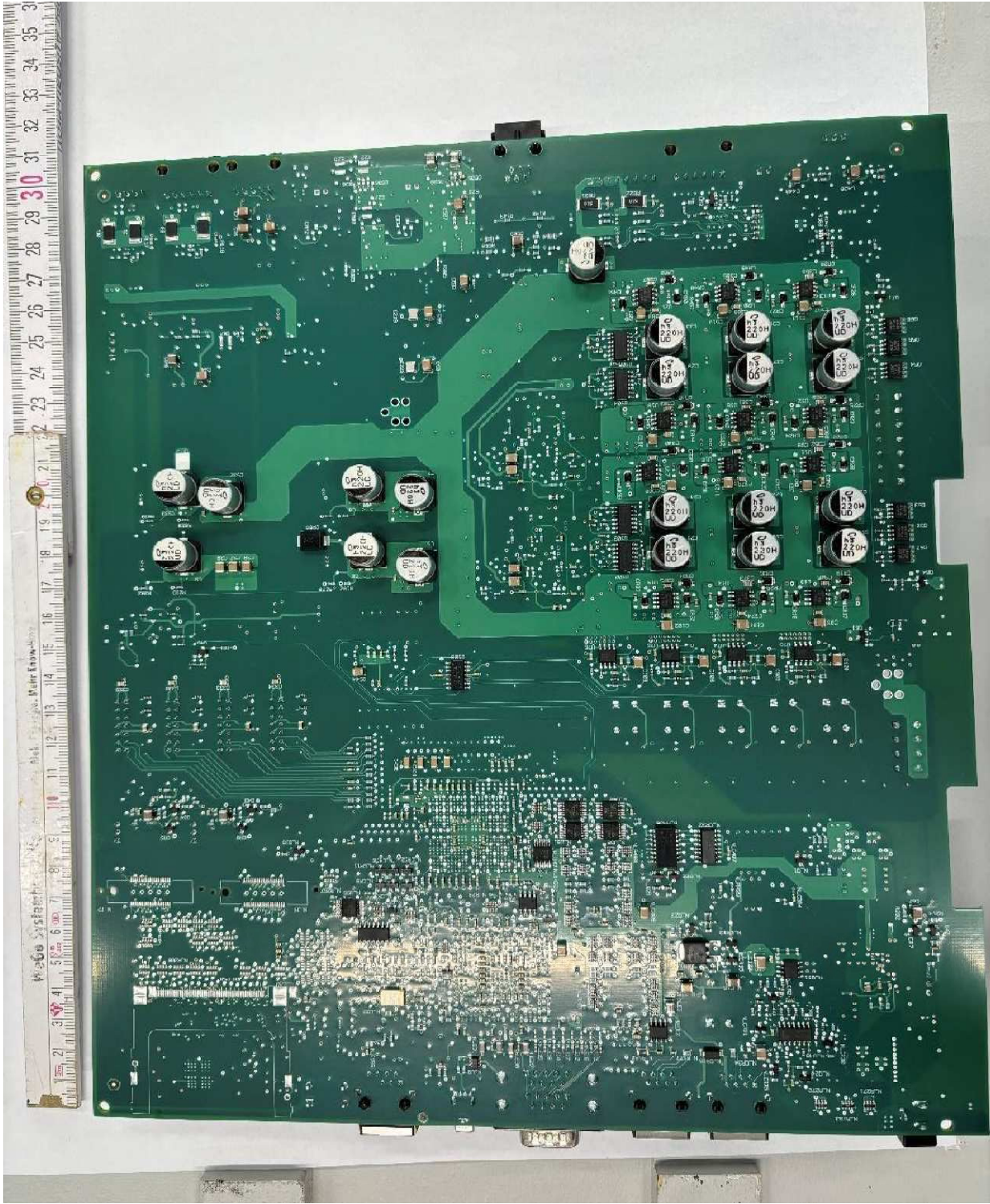
Main-Board bottom
