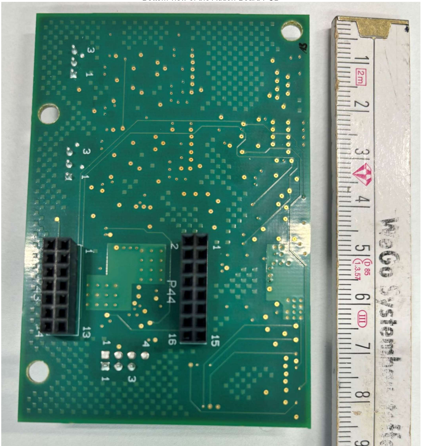
Bottom view of the Addon-Board PCB
