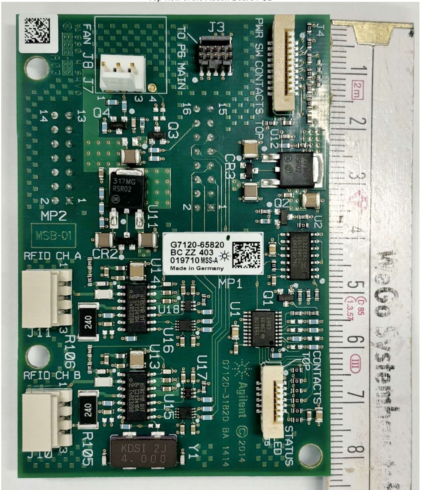
Top view of the Addon-Board PCB
