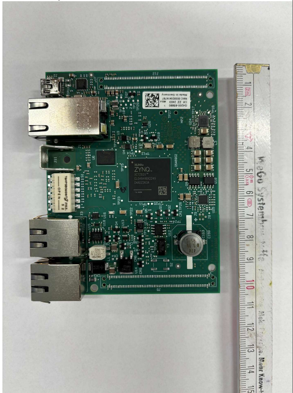
Processor board top
