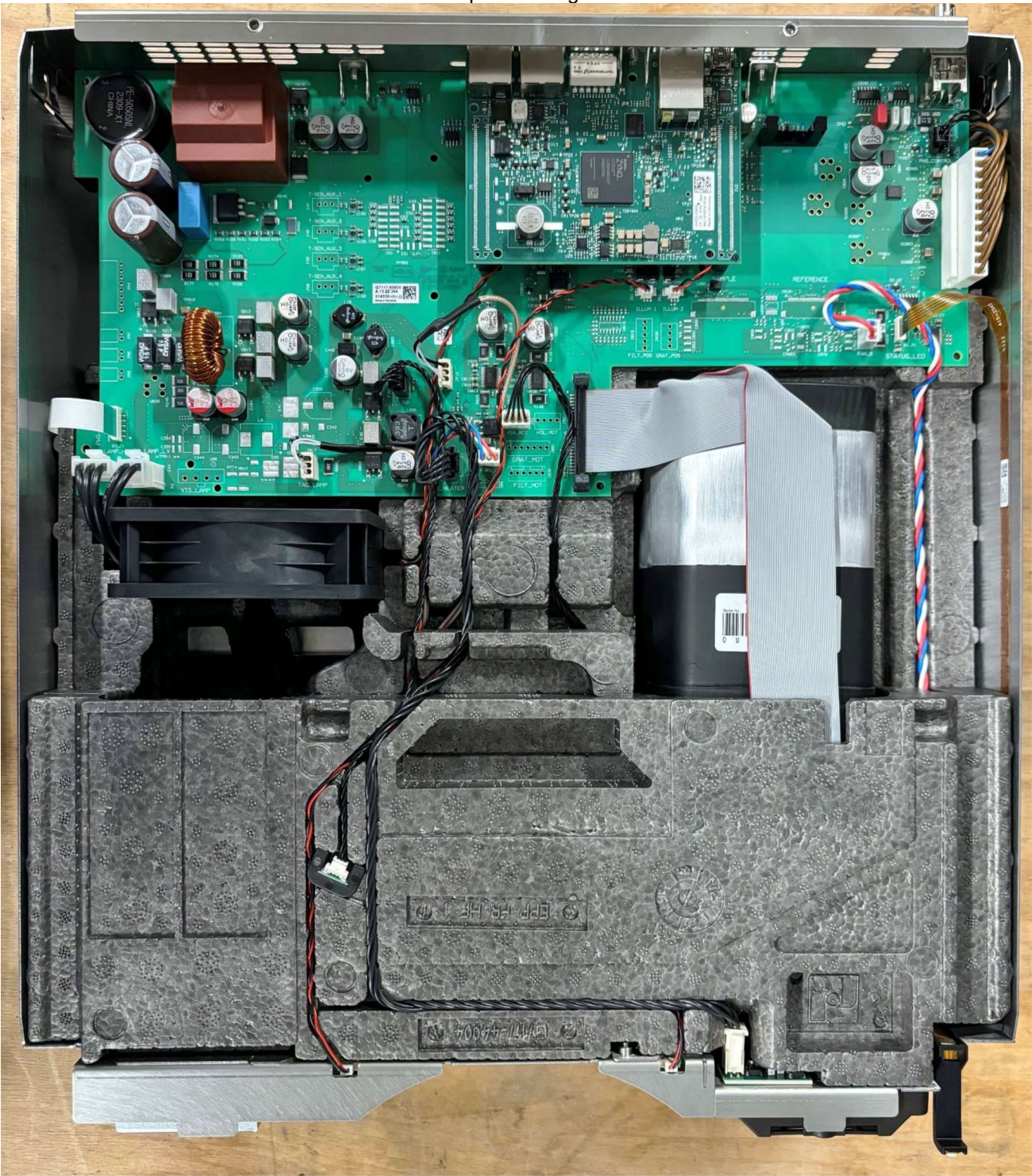
Open housing
