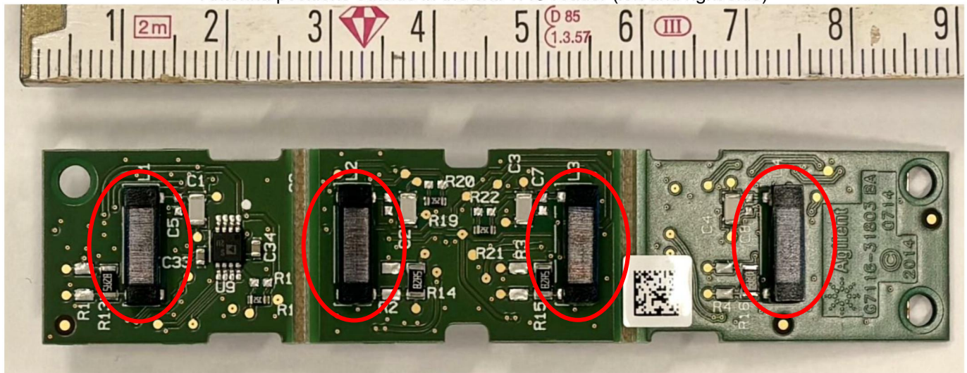
Antenna positions outside in the ext. TAG reader (left and right side)
