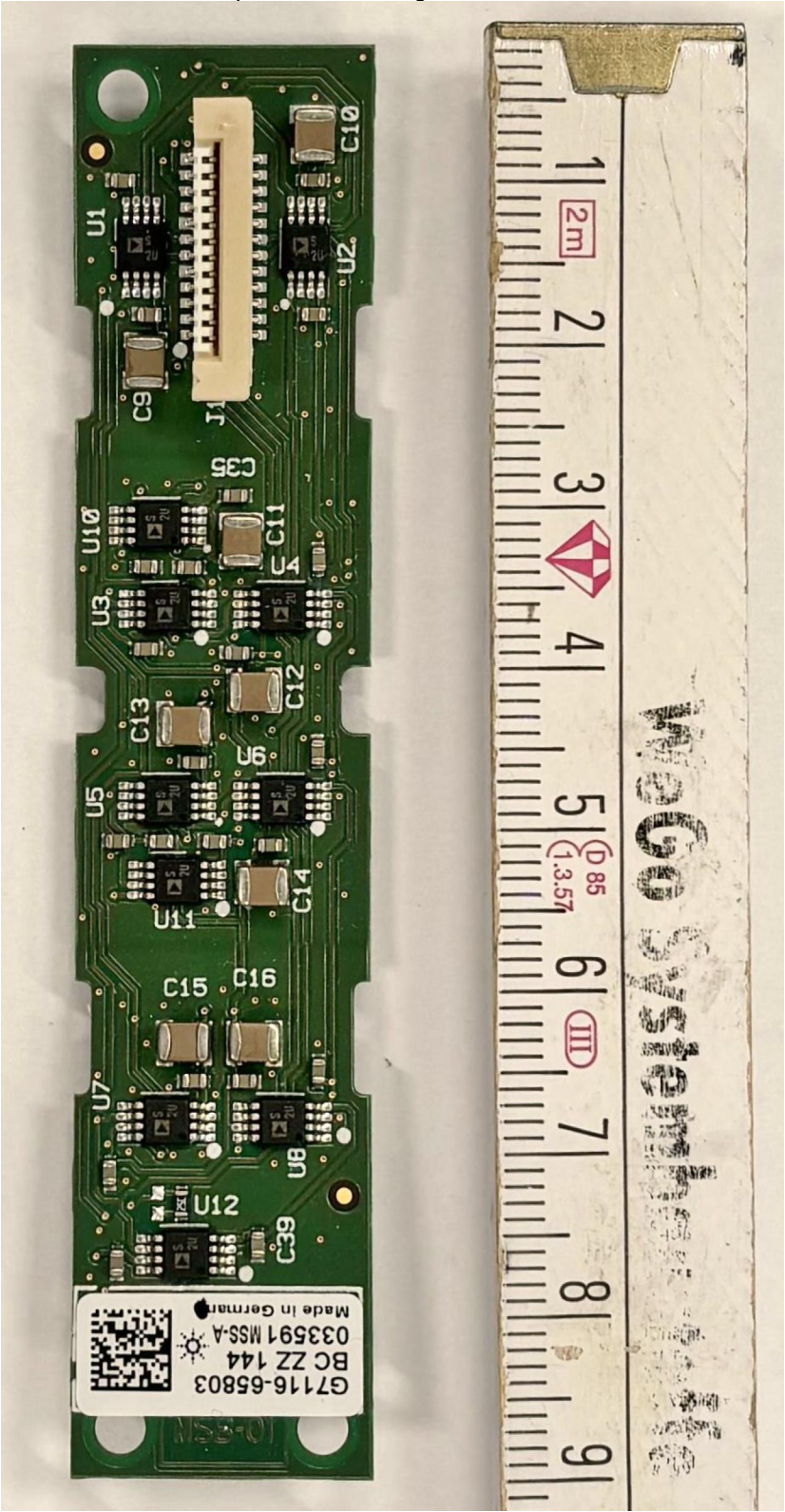
Top view of the Tag-Reader PCB
