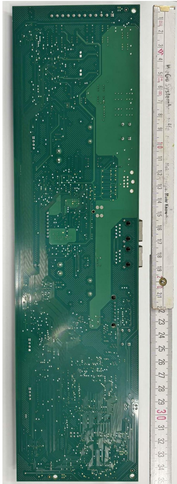
Bottom view of the Main-Board PCB
