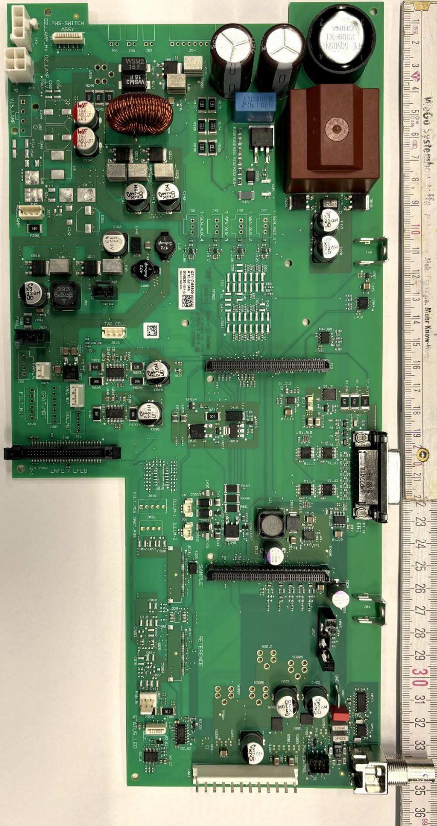
Main-Bord top
