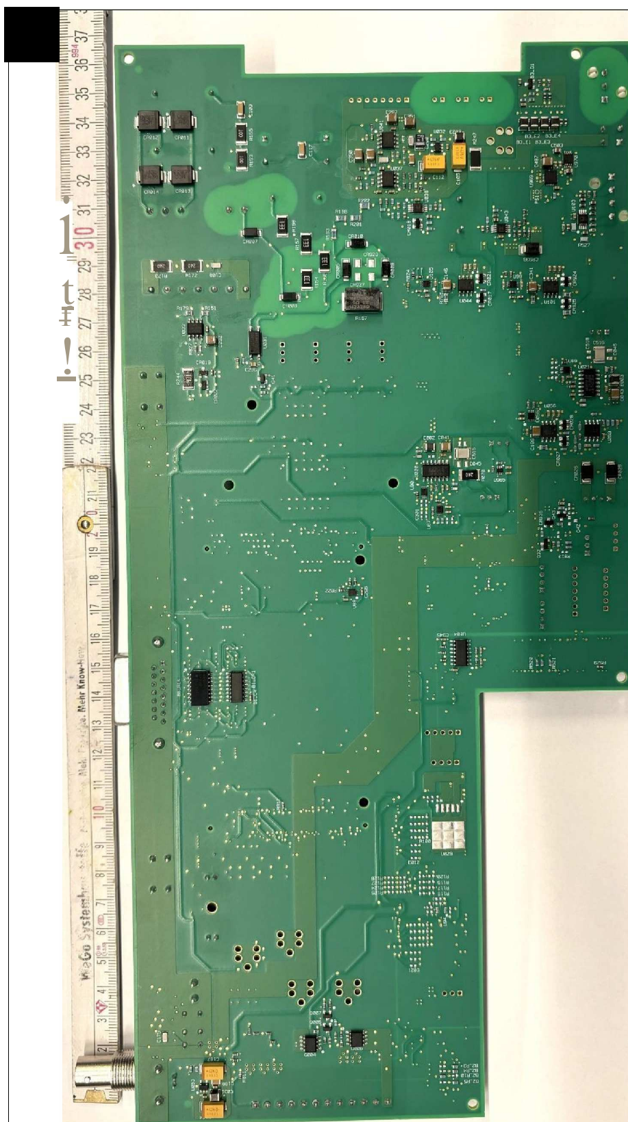
Main-Board bottom
