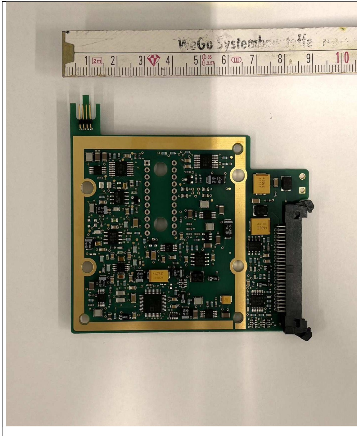
Optics board top
