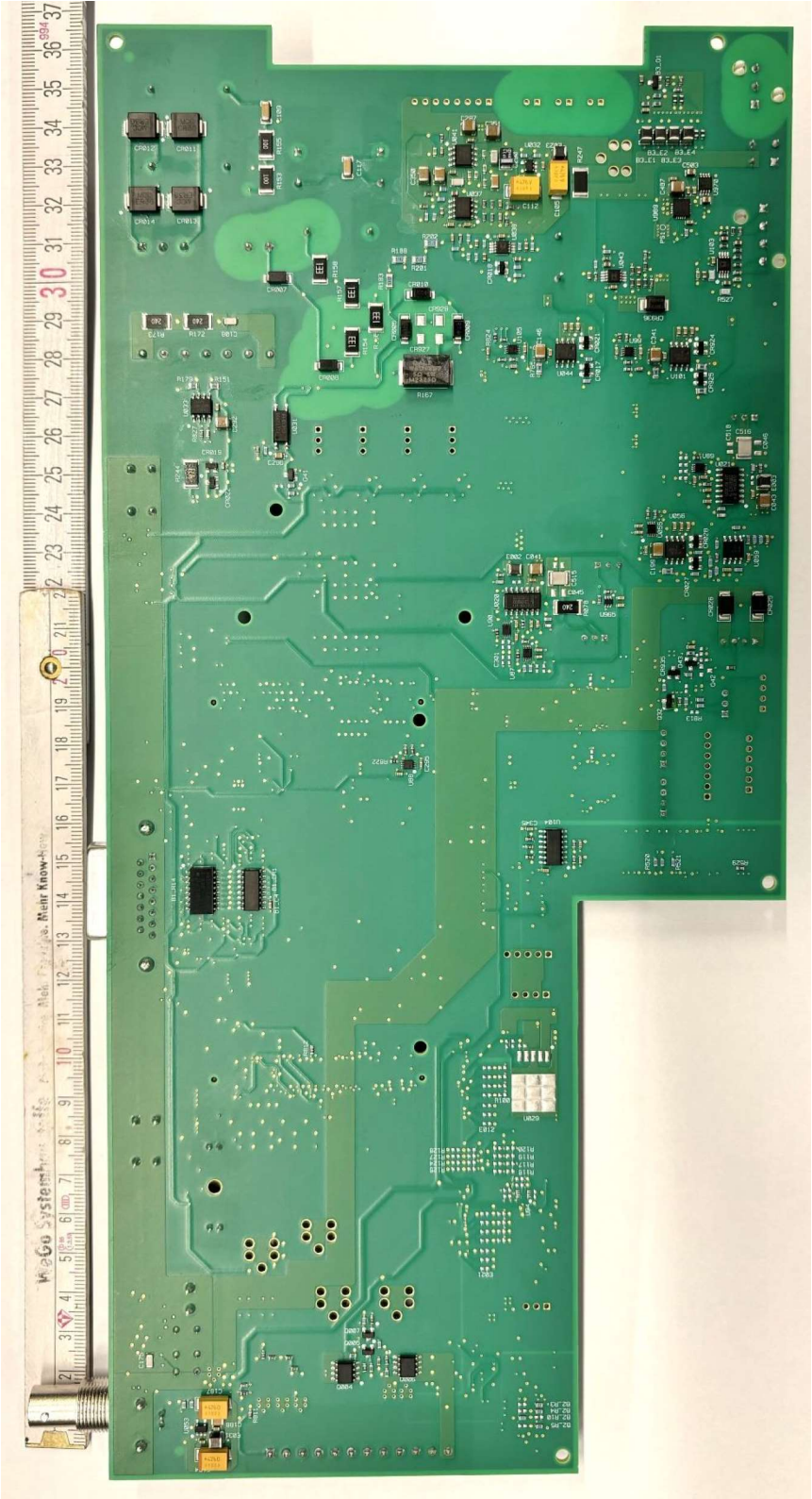
Bottom view of the Main-Board PCB
