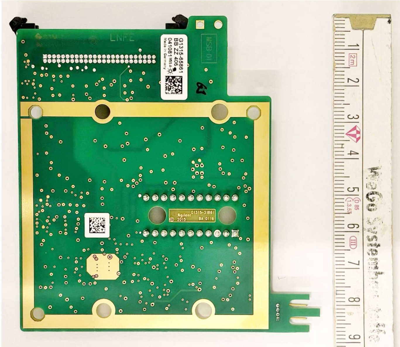
Bottom view of the LNFE-Board PCB
