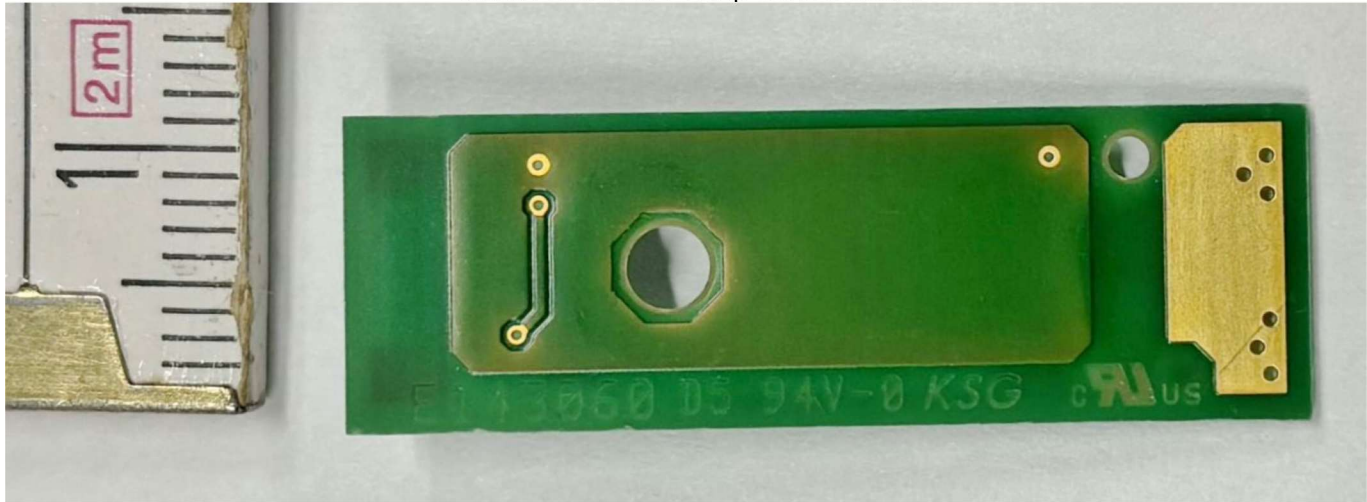
Bottom view of the Temp-Sensor Board
