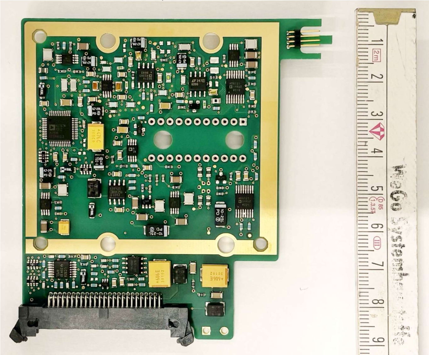
Top view of the LNFE-Board PCB
