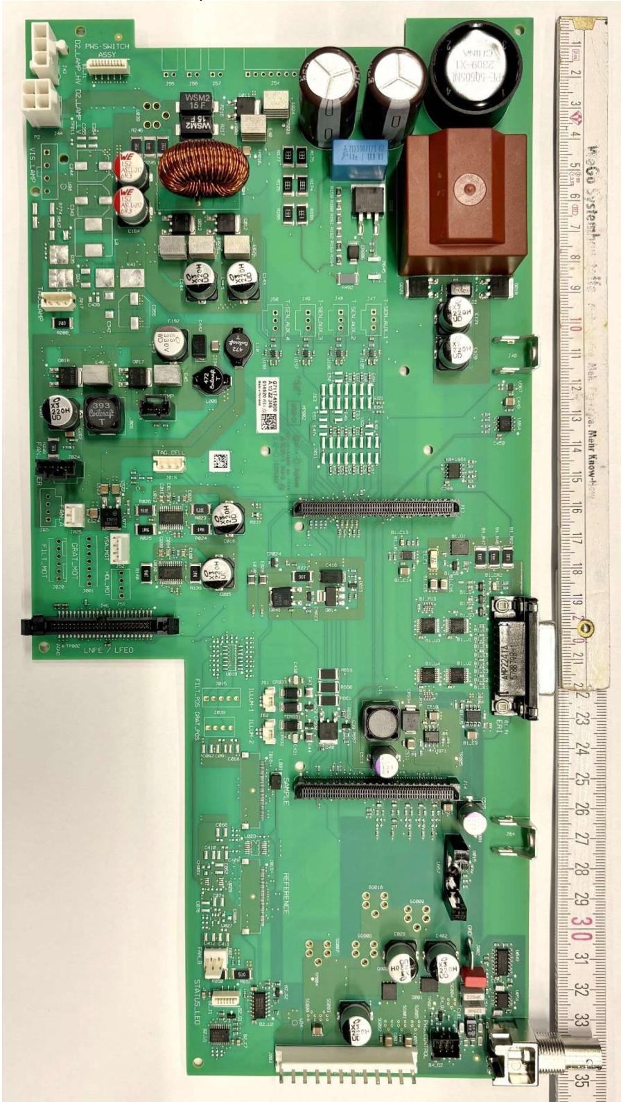
Top view of the Main-Board PCB
