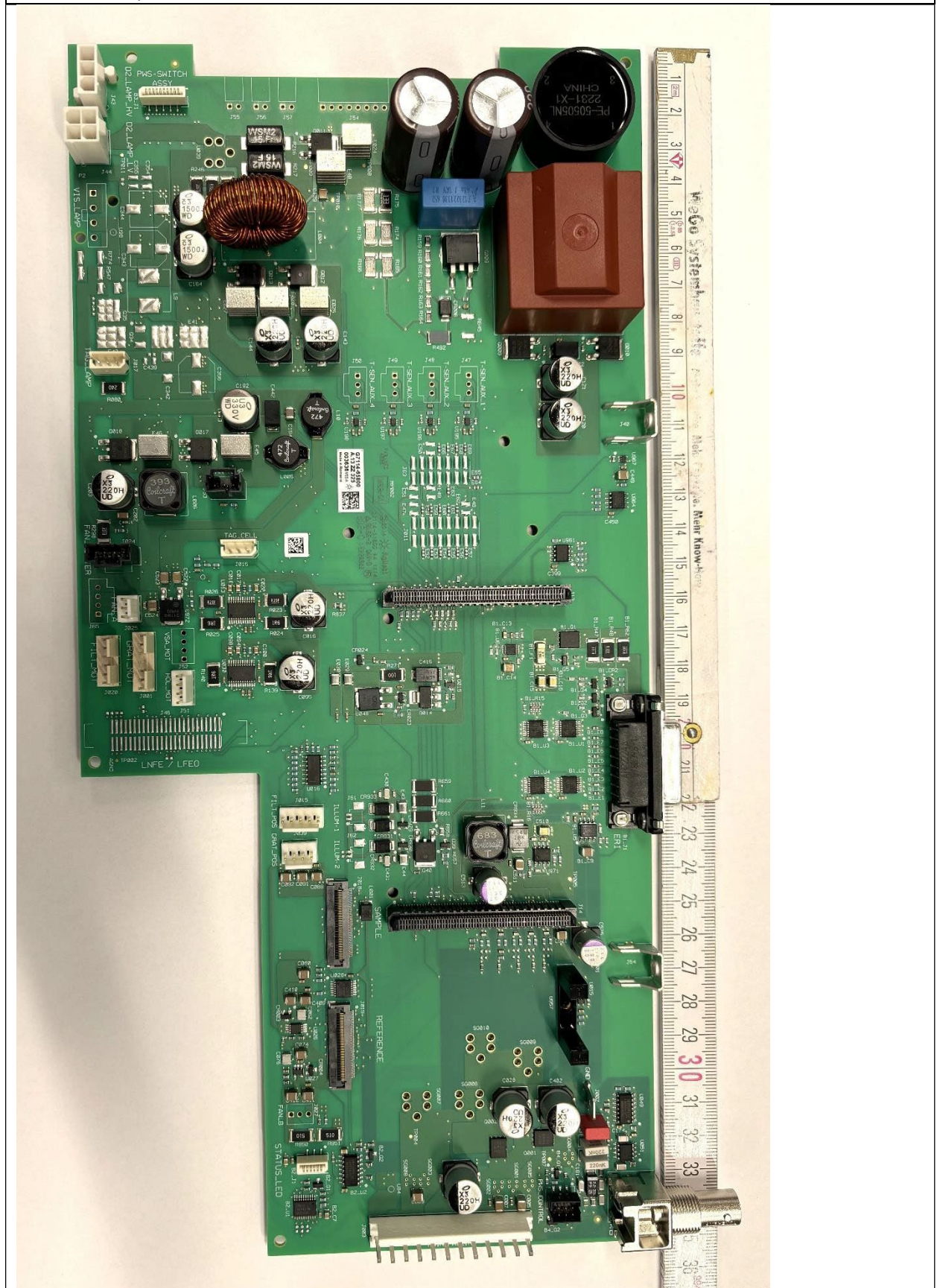
Main-Bord top
