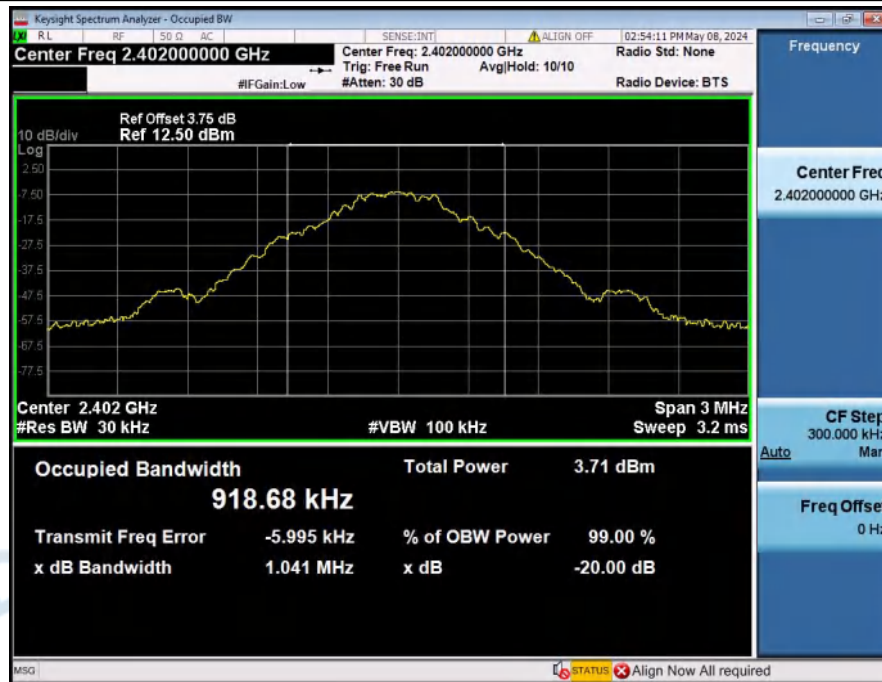
-20dB_Bandwidth_NVNT_ANT1_1-DH5_2402
