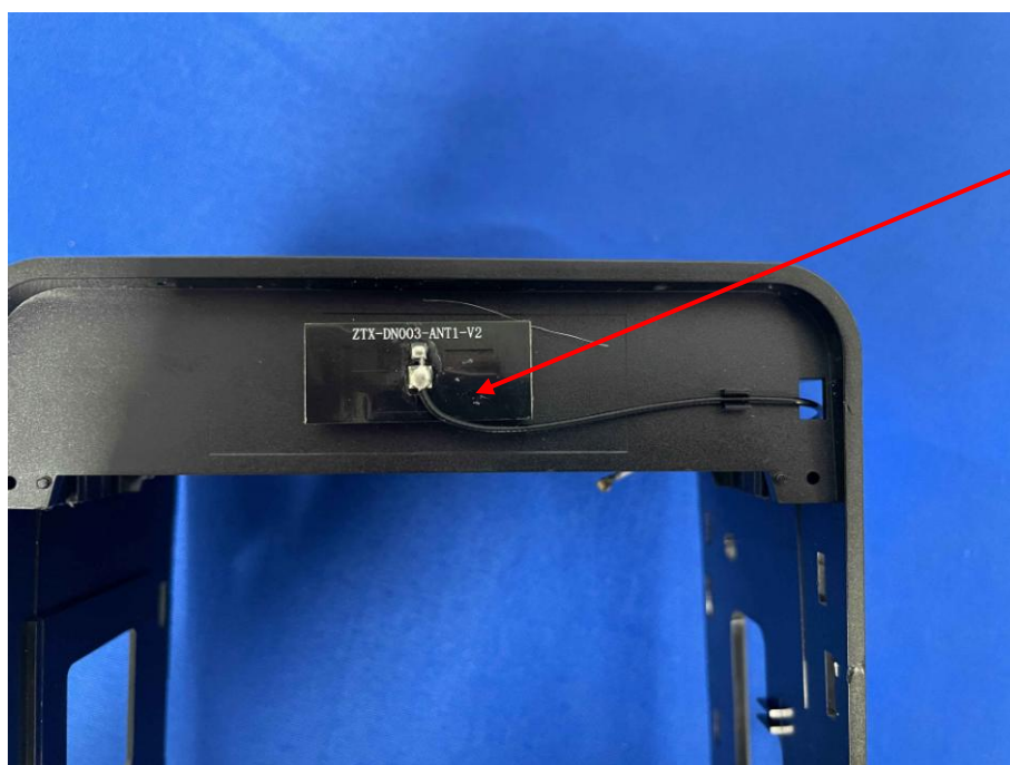
BT/2.4G WIFI/5G WIFI Antenna 1
