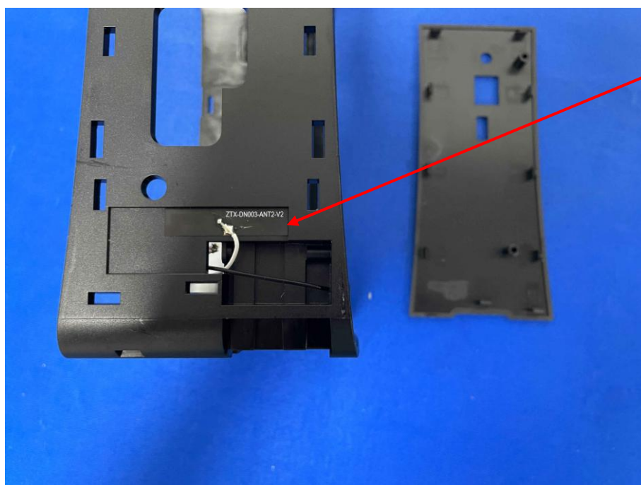
2.4G WIFI/5G WIFI Antenna 2
