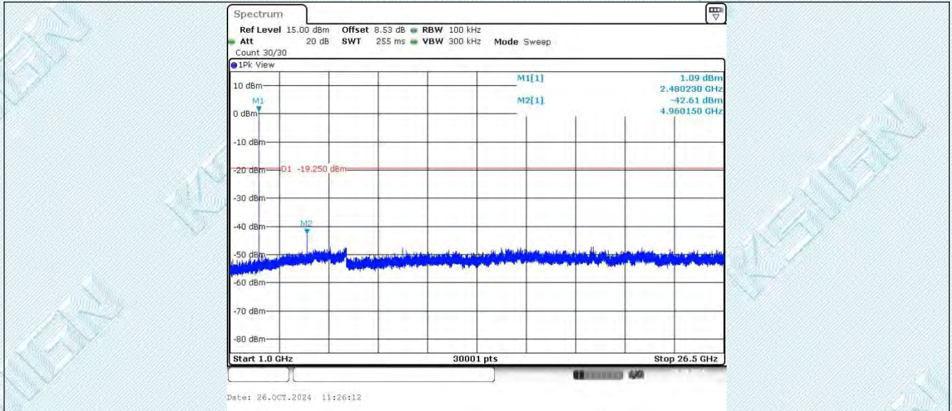
3DH5_Ant1_2402_30~1000
