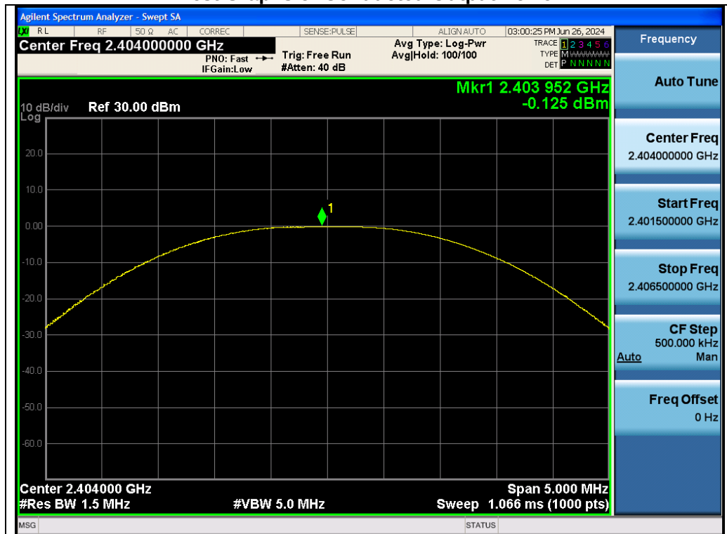
Test_Graph_LE1M_ANT1_2404_1Mbps_Peak Power
