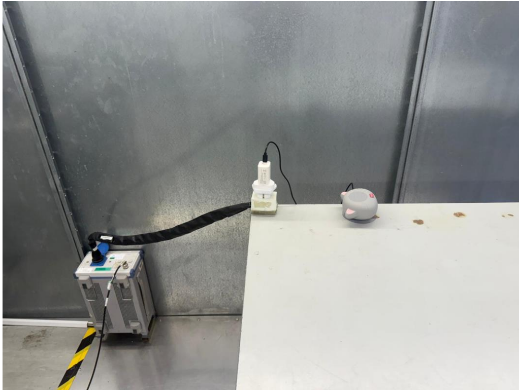
Set up for Conducted Emission on AC Mains
