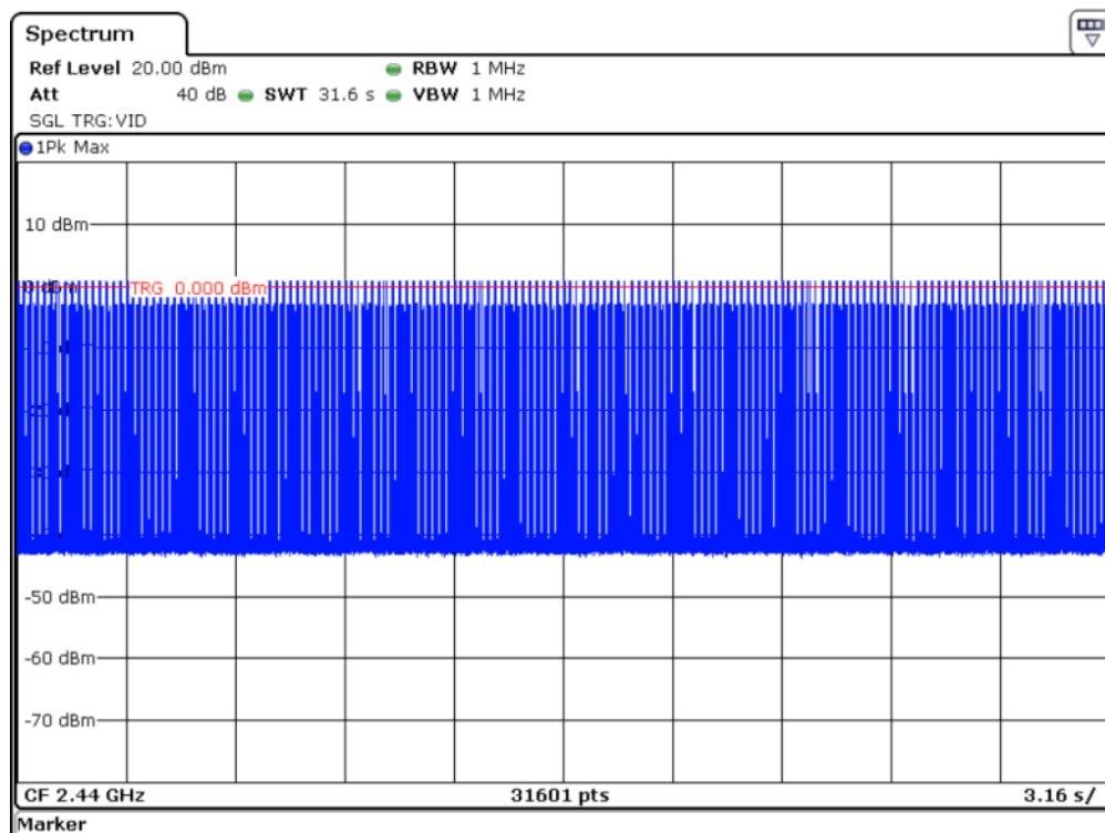
EDR, 2-DH1, Tx frequency: Frequency hopping
