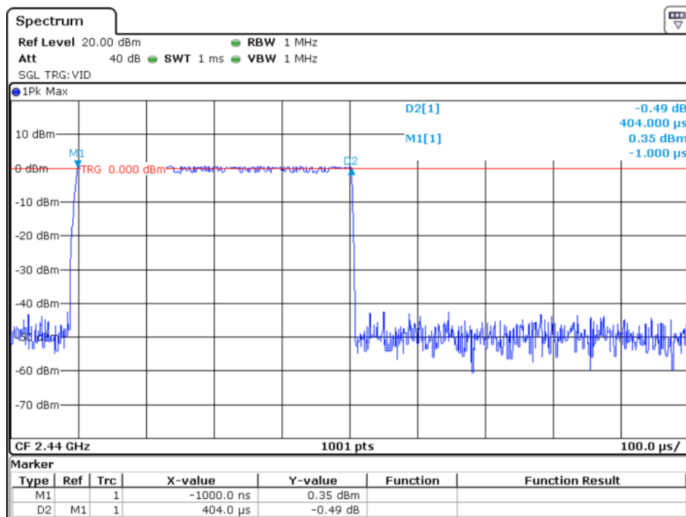
EDR, 2-DH1, Pulse width
